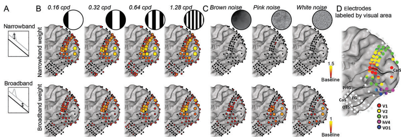
Figure 3. Spatial distribution of narrowband (gamma) and broadband weights. (A) Spectral power changes during visual stimulation compared with baseline were separated in increases in narrowband gamma rhythms and broadband increases by fitting a power law shape with a Gaussian. (B) Spatial distribution of narrowband gamma (top) and broadband weights (bottom) in Subject 1 during grating stimuli. (C) Spatial distribution of narrowband gamma (top) and broadband weights (bottom) in Subject 1 during noise stimuli. Electrodes that showed a significant increase compared with baseline are plotted in color on the rendered brain surface ( P < 0.05 uncorrected). (D) ECoG electrodes labeled by visual field mapping experiment (Winawer et al. 2013). CalS = calcarine sulcus, PHG = parahippocampal gyrus, CoS = collateral sulcus, FG = fusiform gyrus, and OTS = occipital-temporal sulcus.
