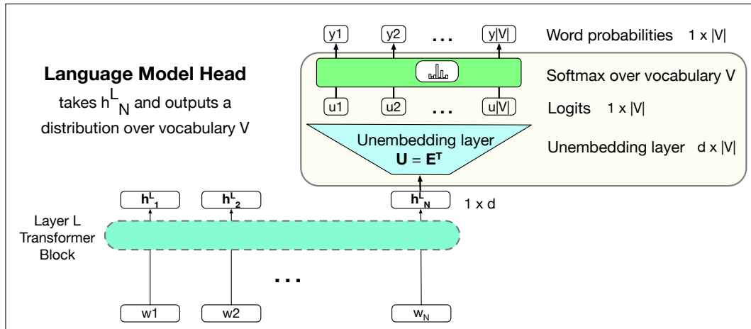
Figure 9.14 The language modeling head: the circuit at the top of a transformer that maps from the output embedding for token N from the last transformer layer ( \mathbf{h}_N^L ) to a probability distribution over words in the vocabulary V .
