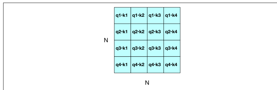
Figure 9.8 The N \times N \mathbf{QK}^{\mathbf{T}} matrix showing how it computes all q_i \cdot k_j comparisons in a single matrix multiple.
