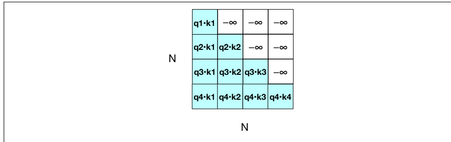
Figure 9.9 The N \times N \mathbf{Q}\mathbf{K}^T matrix showing the q_i \cdot k_j values, with the upper-triangle portion of the comparisons matrix zeroed out (set to -\infty , which the softmax will turn to zero).
