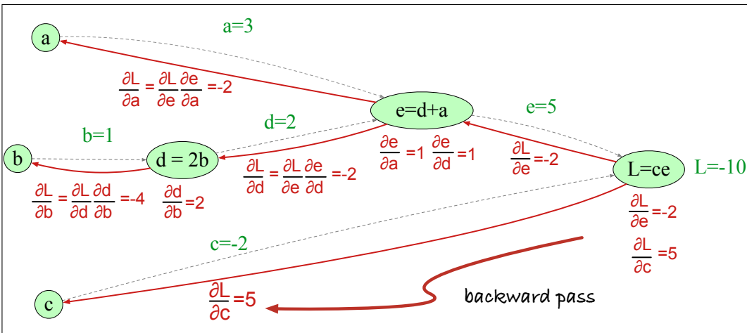
Figure 7.14 Computation graph for the function L(a,b,c) = c(a+2b) , showing the backward pass computation of \frac{\partial L}{\partial a} , \frac{\partial L}{\partial b} , and \frac{\partial L}{\partial c} .
