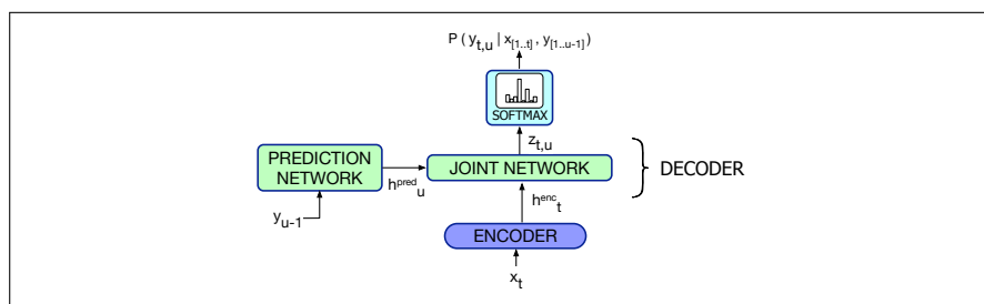
Figure 16.14 The RNN-T model computing the output token distribution at time t by integrating the output of a CTC acoustic encoder and a separate ‘predictor’ language model.
