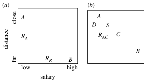
Figure 10. Configurations of alternatives in the attribute space. In each panel, the two axes denote two attributes of the alternatives (sample attributes' labels are given in (a)). The capital letters denote the positions of the alternative choices in the attribute space, while letters R_i denote the reference points. (a) Reference effect in multi-attribute decision making (after Tversky & Kahneman 1991). (b) Contextual preference reversal: the similarity, attraction and compromise effects. Alternatives A, B, C and S lie on the indifference line.
