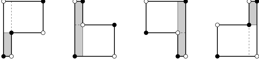
FIGURE 26. The four cases in Lemma 4.12. Each case is a decomposition r_1 * r_2 , where r_1 is shown shaded. The dotted line gives the alternate decomposition r_1' * r_2' .
