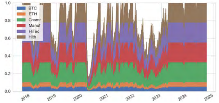
(a) EWMA volatility estimator.
