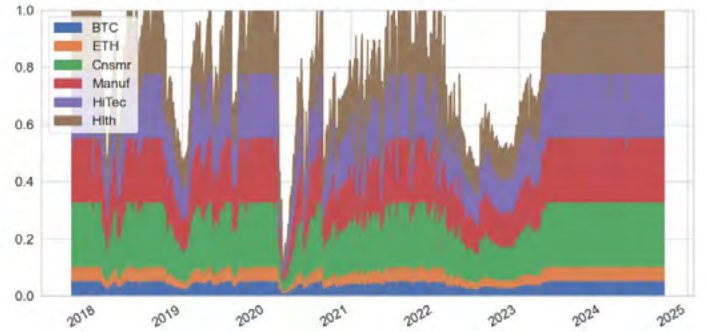
(b) GARCH volatility estimator.
