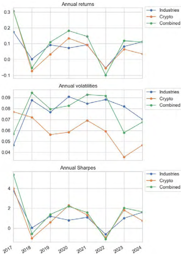
Figure 8: Annual performance metrics of the three portfolios.
