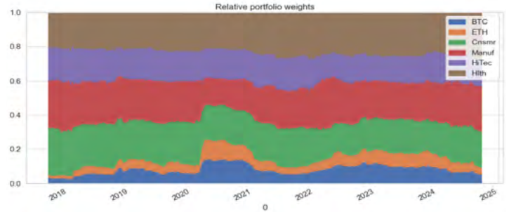
Figure 9: Relative weights of the combined portfolio.
