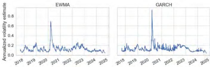
Figure 10: Annualized volatility estimates of the 90/10 portfolio.
