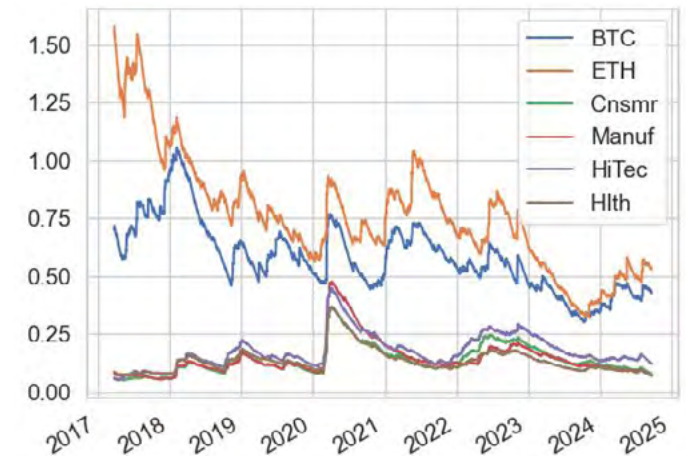
Figure 4: Estimated annualized volatilities of the six assets.
