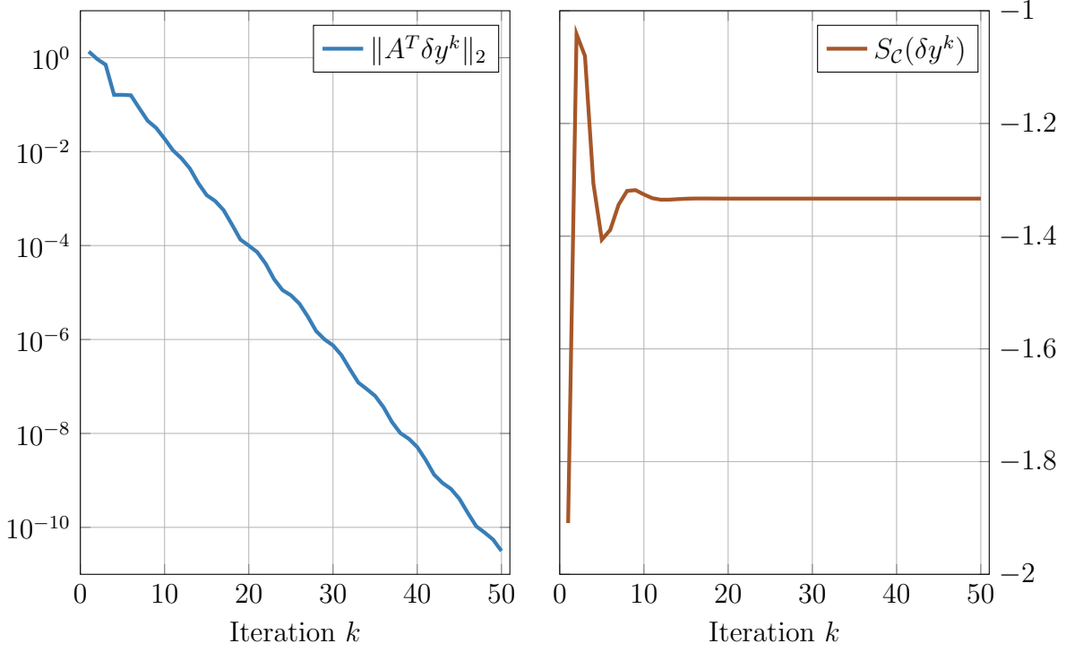
Figure 2: Convergence of \{\delta y^k\}_{k \in \mathbf{N}} to a certificate of primal infeasibility for problem (26) with a = 1 , u_1 = 0 and u_3 = 3 .
