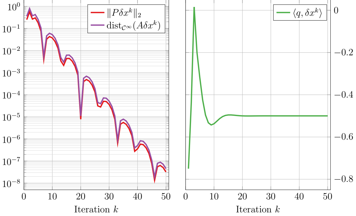
Figure 3: Convergence of \{\delta x^k\}_{k \in \mathbf{N}} to a certificate of dual infeasibility for problem (26) with a = 0 , u_1 = 2 and u_3 = +\infty .
