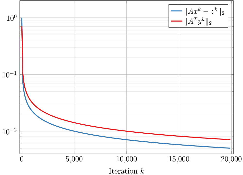
Figure 7: Convergence of residuals \|Ax^k - z^k\|_2 and \|A^T y^k\|_2 for problem (28).
