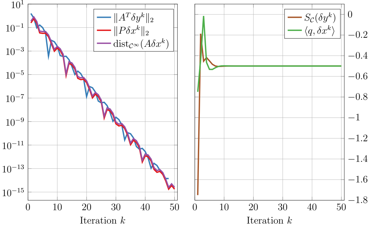
Figure 4: Convergence of \{\delta y^k\}_{k \in \mathbb{N}} and \{\delta x^k\}_{k \in \mathbb{N}} to certificates of primal and dual infeasibility, respectively, for problem (26) with a = 0 , u_1 = 0 and u_3 = +\infty .
