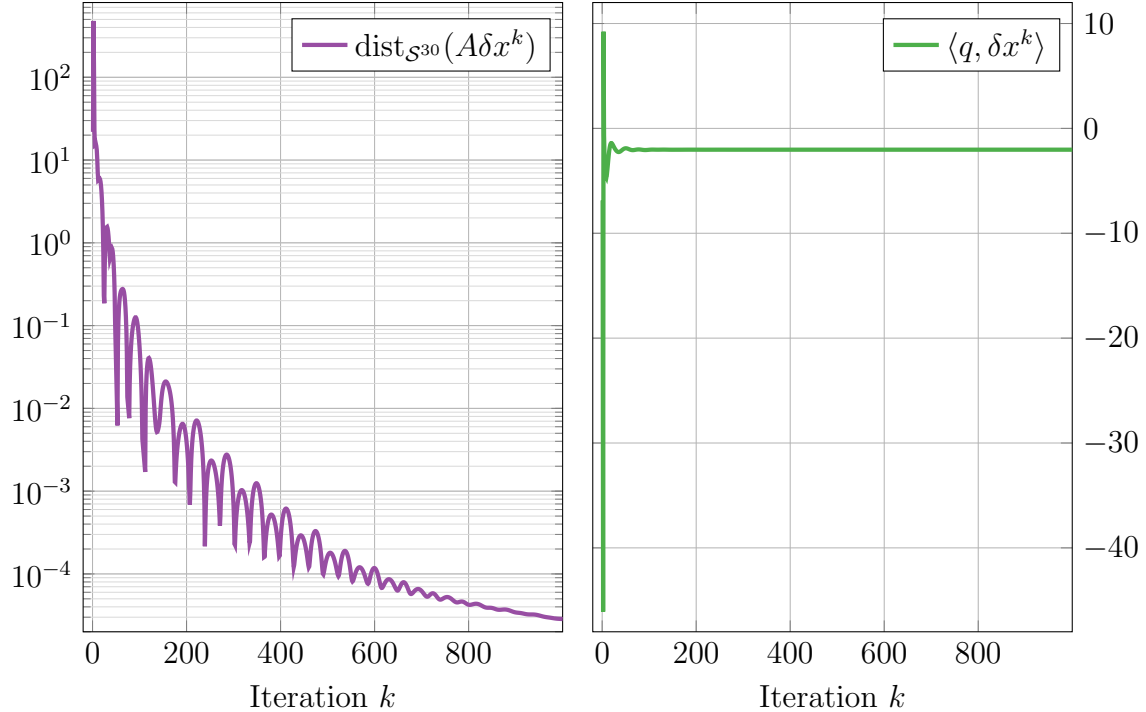
Figure 6: Convergence of \{\delta x^k\}_{k \in \mathbb{N}} to a certificate of dual infeasibility for problem infd1 from SDPLIB.
