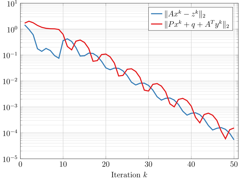
Figure 1: Convergence of \{x^k, z^k, y^k\}_{k \in \mathbb{N}} to a certificate of optimality for problem (26) with a = 1 , u_1 = 5 and u_3 = 3 .
