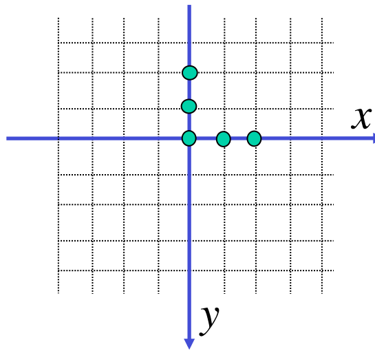
\Pi_{xy}
