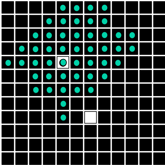
f[x, y]
