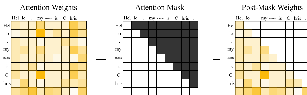
Figure 4: Example of causal masking in multi-headed self-attention before softmax normalization.
