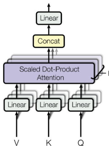
Multi-Head Attention
