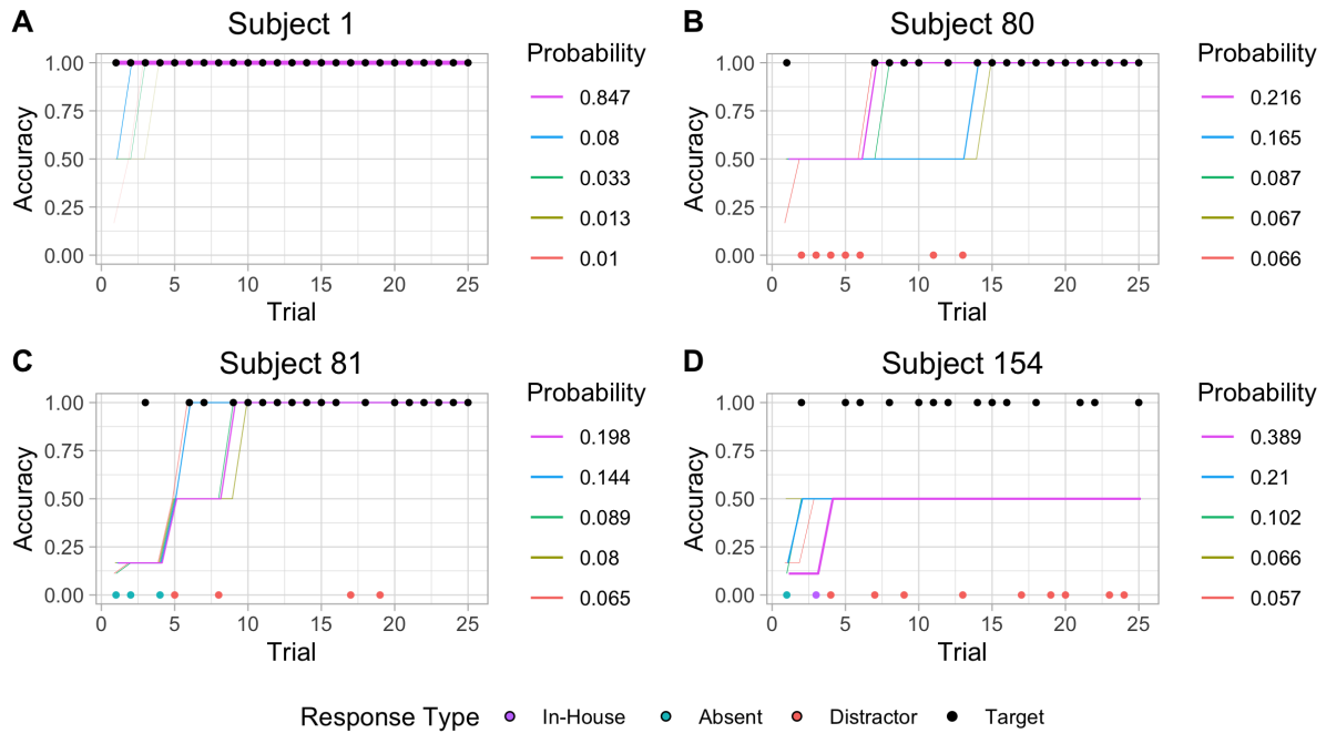
Figure 4: Responses of selected solvers (panels a-c) and one non-solver (panel d) during the practice phase and their top 5 Viterbi paths from individually fitted HMMs according to their posterior probabilities. Target (correct) responses are placed at accuracy of 1 whereas incorrect responses are placed at 0. Viterbi path lines are placed horizontally at positions corresponding to the probability that responses based on the strategy will be correct, e.g. successful at 1 and prevalent digits at 0.5, ignoring strategy execution errors. Line thicknesses indicate path posterior probabilities. The fit to the non-solver used an HMM based on aggregate response profiles of non-solvers. See SI Section 4.1.
