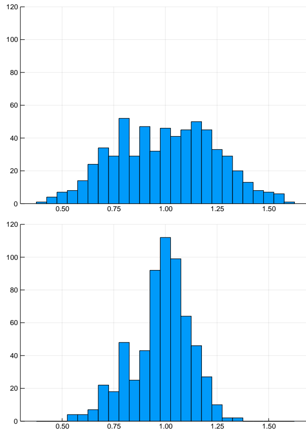
Figure 12.1 Histogram of pixel illumination values using p = 1 (top) and \hat{p} (bottom). The target intensity value is one.
