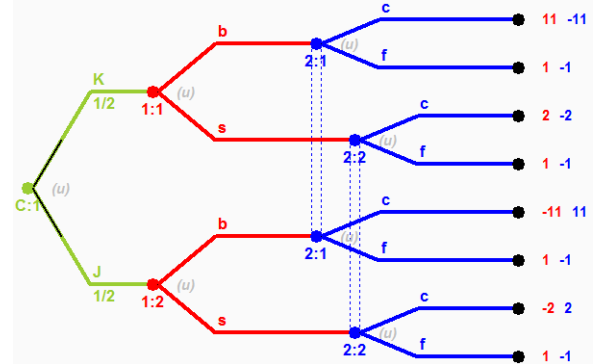
Fig. 1. Chance deals player 1 king or jack with probability \frac{1}{2} at the green node. Then player 1 selects big or small bet at a red node. Then player 2 chooses call or fold at a blue node.
