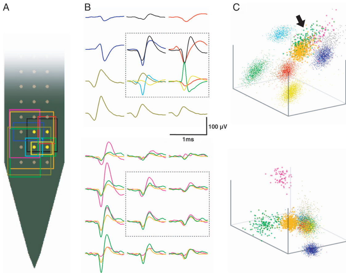
FIG. 3. Polytrodes provide better single-unit isolation than tetrodes. A : breaking the polytrode into “virtual tetrodes” revealed that 7–24 neurons were recorded on any one virtual tetraode of a 54\mu\text{m} \times 1\text{b} polytrode. In the example shown here (highlighted sites), 10 neurons were identified, their approximate field sizes represented by the colored boxes. B : spike waveforms of these 10 neurons, 7 of which were isolatable using the tetraode sites alone ( top boxed region ) and 3 that could only be isolated by including spike waveforms from the surrounding recording sites ( bottom ). Note the similarity of the spike shapes and amplitudes on the tetraode sites. C : a tetraode-derived cluster plot ( top ) shows 5 of the 7 well-isolated neurons. Whereas 2 other neurons (black and gold dots) were separable along other dimensions, 3 neurons (arrow: green, orange, and pink + symbols) were not distinguishable on any projection or hyperplane of the tetraode. Only by incorporating spike waveform indices from the surrounding sites was it possible to cluster and isolate these neurons ( bottom ).
