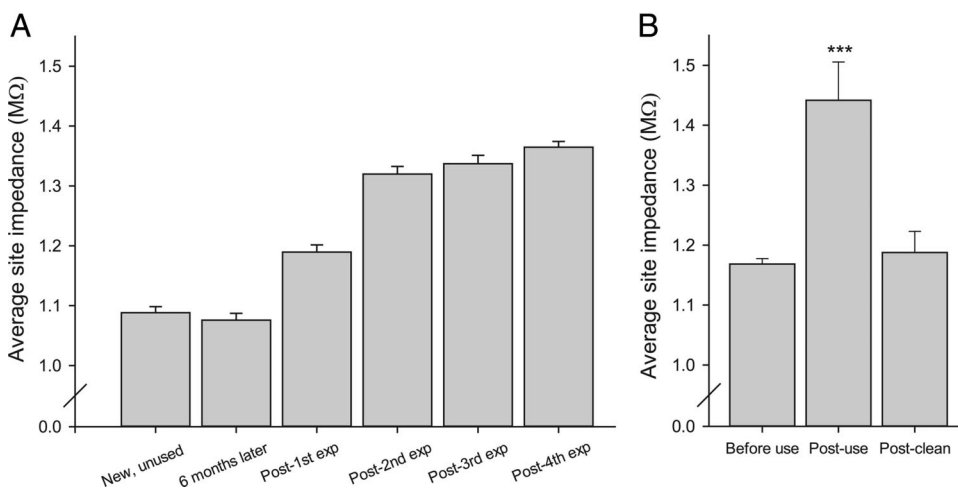
FIG. 4. Long-term stability of recording sites. A : post fabrication site impedances were highly consistent and remained unchanged for 6 mo when stored in air. Over the course of several cat experiments with multiple penetrations in each experiment, site impedances increased slightly; however, recording properties remained similar. B : site impedances of another polytrode, before use, after 5 recording sessions, and after overnight cleaning in trypsin ( ***P < 0.0005 ). Error bars are SE.
