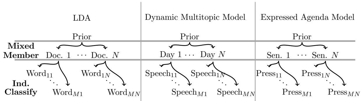
Figure 2: A Common Structure Across Seemingly Unrelated Text Models: In each case the mixed member allows the scholar to estimate the parameter of particular substantive interest. The prior facilitates the borrowing of information across units, and the individual elements classified form the observed data.
