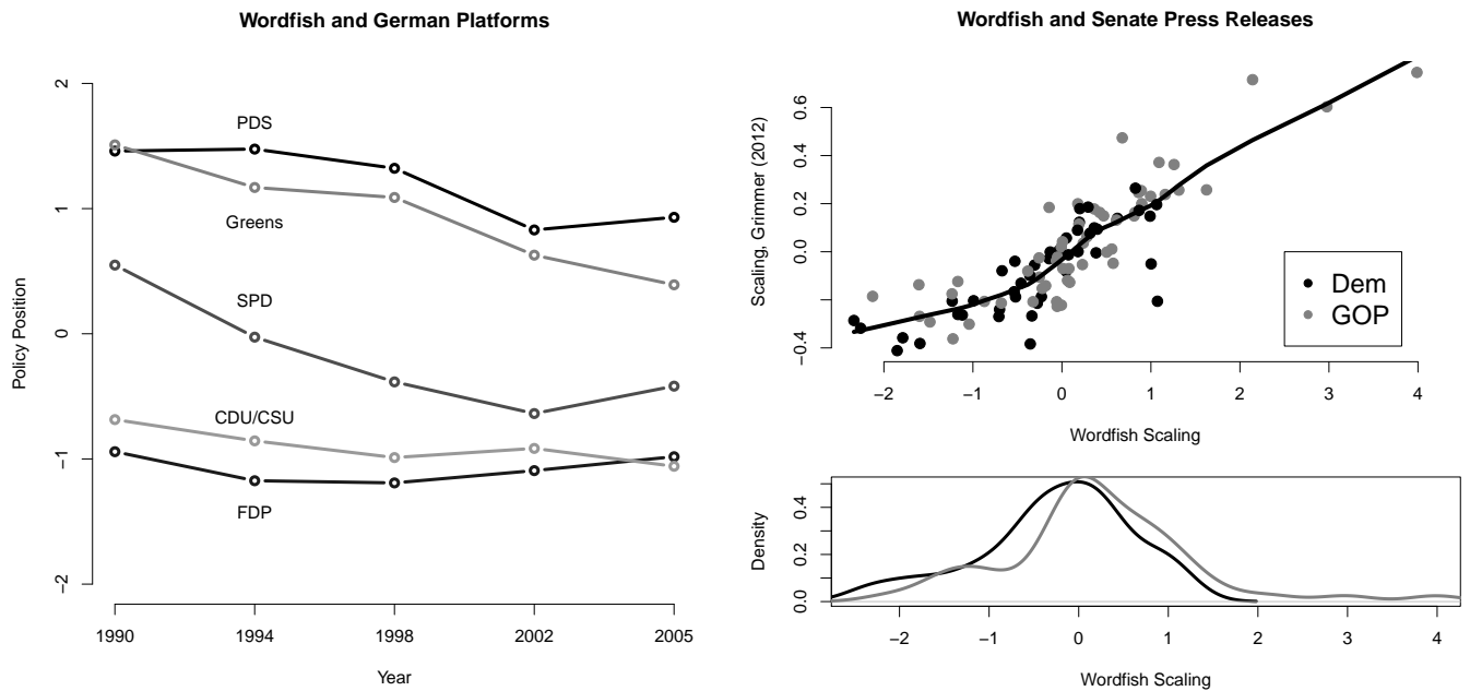
Figure 7: Wordfish Algorithm: Performance Varies Across Context
