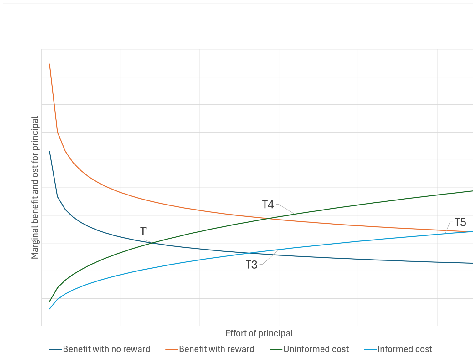
Figure 3: Simulation of equilibrium effort by treatment
