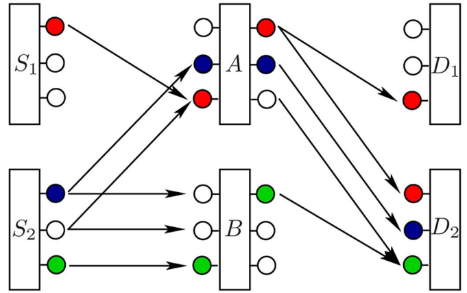
Fig. 2. Deterministic network.
