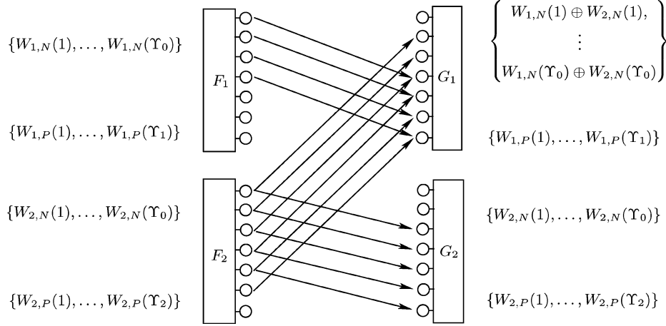
Fig. 14. Deterministic \mathcal{Z} -neutralization network with the message demands.
