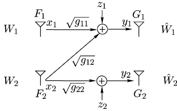
Fig. 9. Gaussian Z network.
