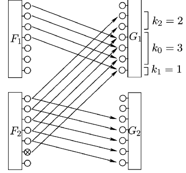
Fig. 19. Deterministic \mathcal{Z} -neutralization network. The upper 2 sub-nodes in G_1 are only connected to F_2 , and, therefore k_2 = 2 . The next 3 sub-nodes receive information from both F_1 and F_2 , and hence, k_0 = 3 . Although the lowest sub-node is also connected to both transmitters, it only receives information from F_1 since F_2 keeps silent on its sub-nodes below n_{22} .
