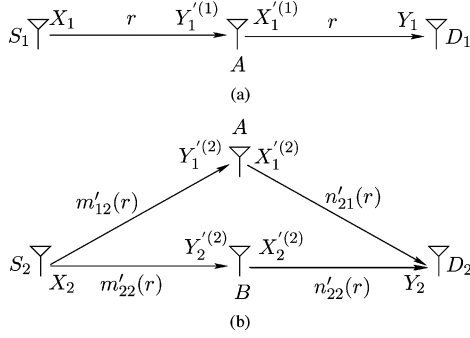
Fig. 13. Effective separated ZS network. (a) Effective channel for $(S_1, D_1)$. (b) Effective channel for $(S_2, D_2)$.
