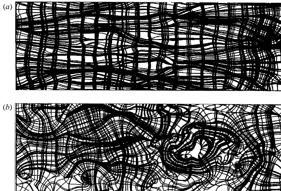
FIGURE 17. Skin-friction lines and surface vorticity lines superimposed. (a) Unseparated region. (b) Separated region.
