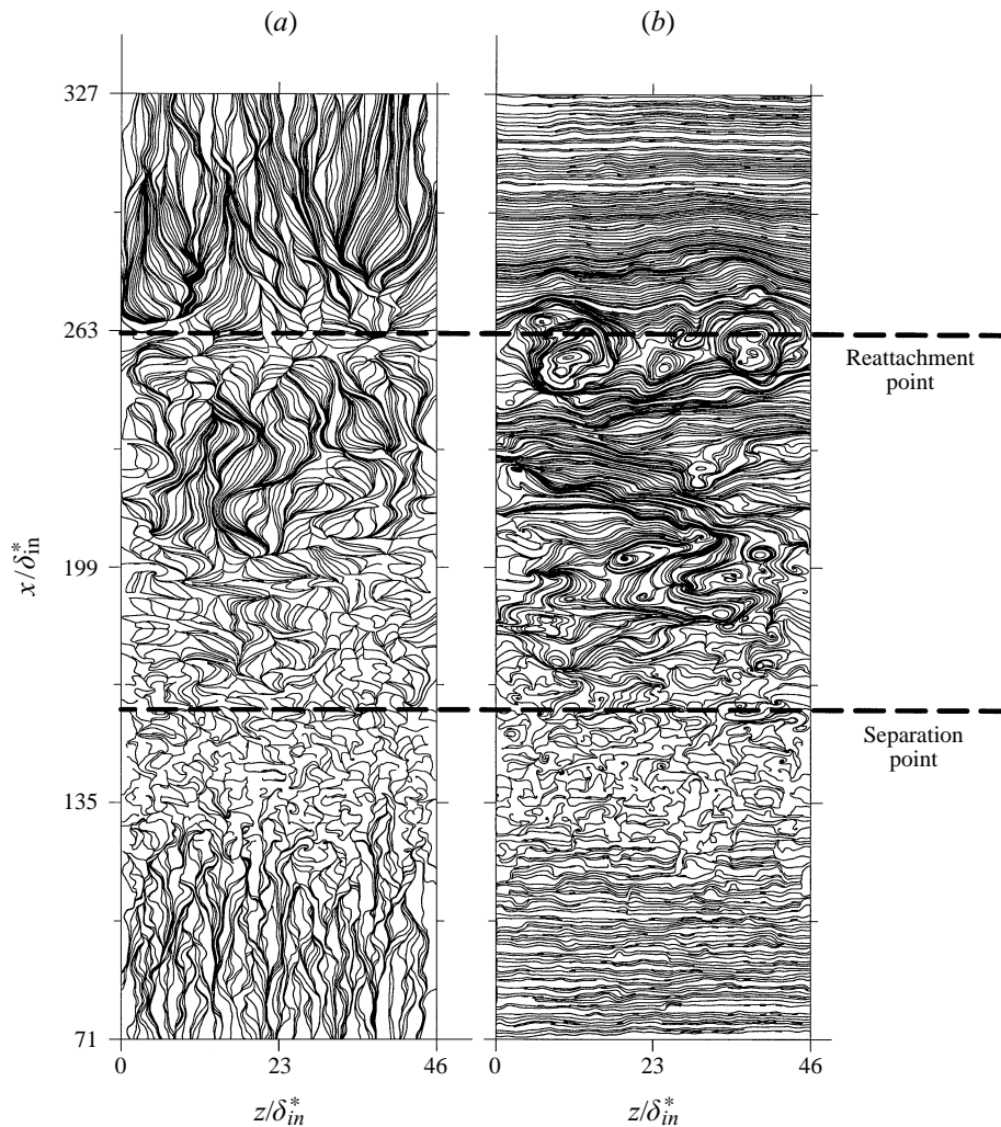
FIGURE 16. (a) Skin-friction lines and (b) surface vorticity lines from x/\delta_{in}^* \approx 90 to x/\delta_{in}^* \approx 300 .
