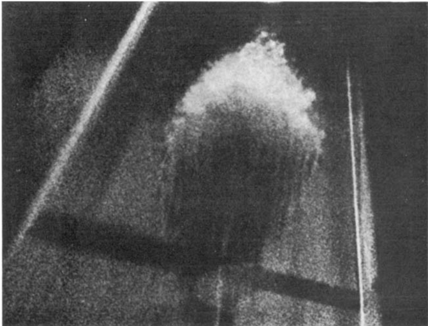
FIGURE 5. Smoke visualization of turbulent spots in air (courtesy of M. R. Head). (a) Oblique view of spot approaching observer, with illumination by light sheet above laminar boundary layer. (b) Oblique view of spot receding from observer, with more diffuse illumination than in (a).
