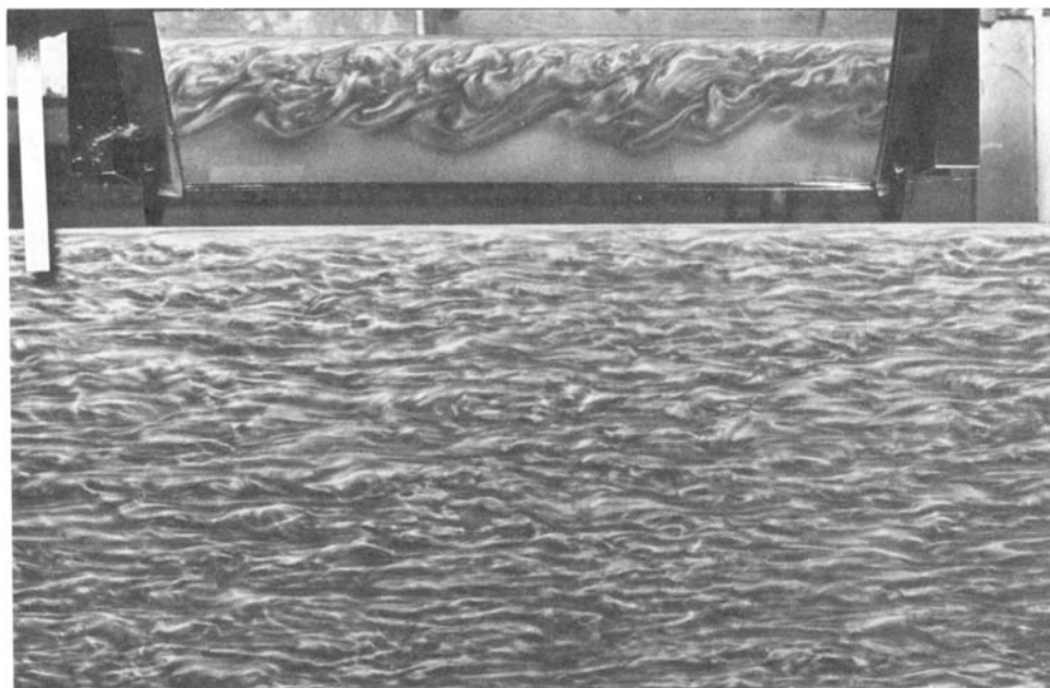
FIGURE 7. Aluminium visualization of sublayer streaks for half-spot and for boundary layer. (a) Half-spot at low Reynolds number; U_\infty = 12 cm/s. Mirror is used to show simultaneous view of free surface. (b) As in (a), but with fully turbulent boundary layer; U_\infty = 15 cm/s.
