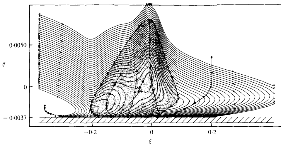
FIGURE 18. Instantaneous streamlines as in figure 17(c) but computed for reference frame moving to right at 0.78U_\infty and also moving upwards at 0.0037U_\infty .
