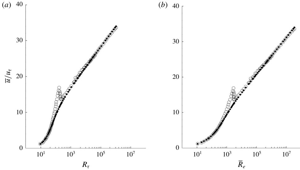
FIGURE 14. (a) Value of \bar{u}/u_\tau versus R_\tau , (b) \bar{u}/u_\tau versus \bar{R}_e . Open circles, ( \circ ) are the combined Oregon and Princeton data from McKeon et al. (2004b). Filled circles ( \bullet ) are computed from (3.5) and (3.13) using (\bar{k}, \bar{a}, \bar{m}, \bar{b}, \bar{n}) = (0.4092, 20.095, 1.621, 0.3195, 1.619) .
