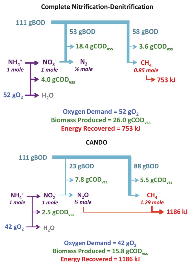
Fig. 8 Comparison of complete nitrification–denitrification to CANDO with respect to oxygen demand, biomass production, and energy recovery.
