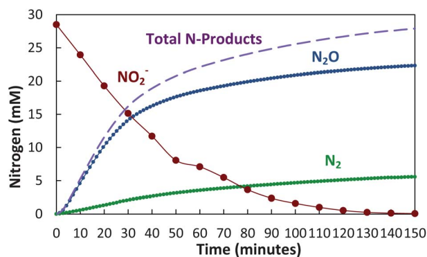
Fig. 2 Reduction of nitrite by carbonate green rust ( \text{Fe}^{\text{II}}_4\text{Fe}^{\text{III}}_2(\text{OH})_{12}\text{CO}_3 ) with over 90% conversion of \text{NO}_2^- to \text{N}_2\text{O} .
