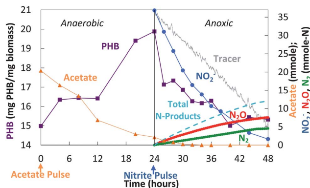
Fig. 5 Decoupled acetate/nitrite addition (cycle 61): changes in acetate, \text{NO}_2^- , \text{N}_2\text{O} , \text{N}_2 , and PHB.
