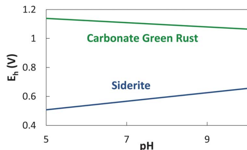
Fig. 1 Redox potential diagram ( E_h vs. pH) for reduction of \text{NO}_2^- to \text{N}_2\text{O} coupled to the oxidation of Fe(II) in siderite and carbonate green rust. Assumed conditions are similar to partially oxidized anaerobic digester centrate: [\text{NO}_2^-] = 35 \text{ mM} , [\text{N}_2\text{O}] = 22 \text{ mM} , [\text{HCO}_3^-] = 40 \text{ mM} . The sources of thermodynamic data were obtained from Rittmann and McCarty for aqueous solutes, 43 see ref. 44 for siderite and ref. 45 for carbonate green rust.
