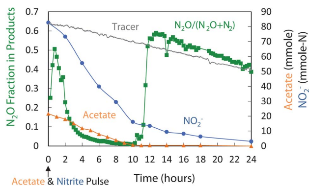
Fig. 3 Coupled acetate–nitrite addition (cycle 107): changes in acetate, \text{NO}_2^- , and \text{N}_2\text{O} production. Of the \text{NO}_2^- consumed, 12% was reduced to \text{N}_2\text{O} , the rest to \text{N}_2 .
