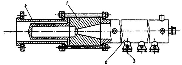
Fig. 5 Schematic of the collector of the hydraulic fire-scale cleaning device using pulsating jets: 1 - cavitation generator; 2 - collector; 3 - nozzles; 4 - filter.
