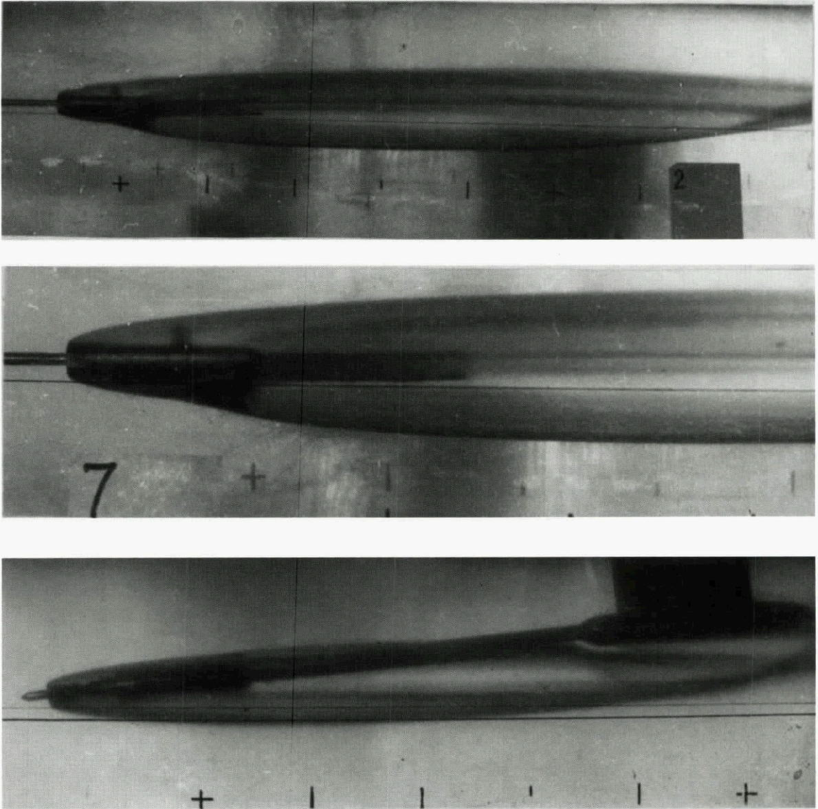
Fig. 5. Cavity in water tunnel.
