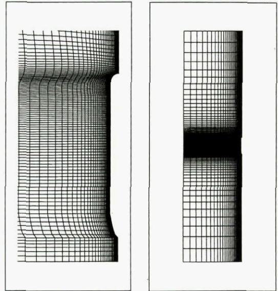
Figure 2 : Mesh of the calculation domain associated a profile having a spherical head
