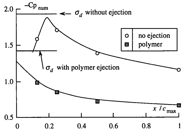
Fig. 7 : Computed pressure coefficient as a function of the downstream distance ( \alpha = 10^\circ , Re = 10^6 ).
