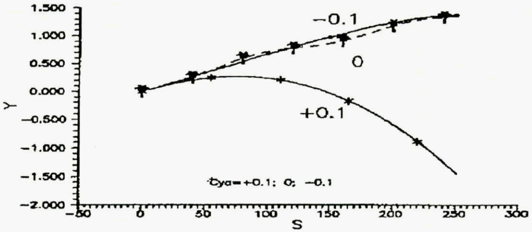
Fig. 8. Influence of C^{\alpha}_{py} on body motion - trajectory
