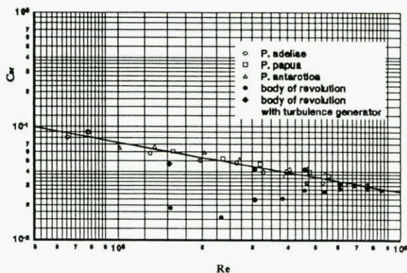
Fig. 4 Frontal drag coefficients plotted against Reynolds numbers. Note that in this graph Re was calculated by using the maximum diameter as reference length.
