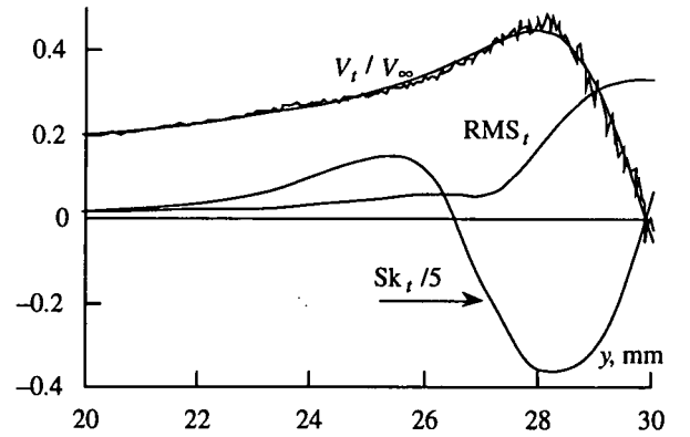
Figure 8 : Adjusted tangential velocity profile at x/c_{\max} = 1 , apparent velocity fluctuation (RMS) and skewness (Sk) distributions due to an assumed excursion of the spatial bias of length equal to 3.8 mm. Free stream velocity 12.5 m/s, polymer solution ejection flow rate 4.7 \text{ cm}^3/\text{s} .
