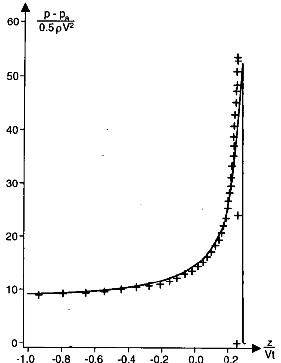
Fig. 7 Prediction of the pressure distribution during water entry of a cone with constant downwards velocity V . Deadrise angle \beta=10^\circ , +, numerical method; —, asymptotic solution.
