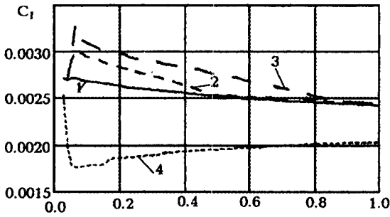
Fig.4. Friction drag coefficient.
