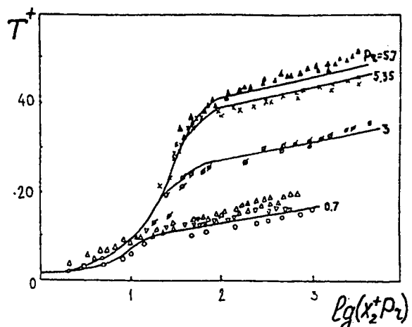
Fig. 2. Comparison of temperature distributions (line) and experimental data of N.M. Galin and P.L. Kirillov [2] for boundary layers on smooth surface with different values of Prandtl number (circles).
