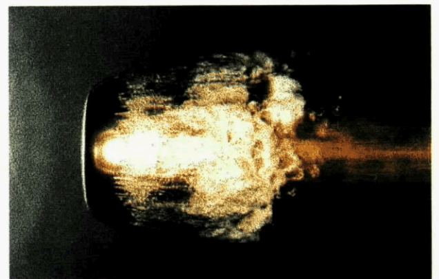
Developed cavitation at \sigma = 0.41 , V_{\infty} = 14.0 m/s
