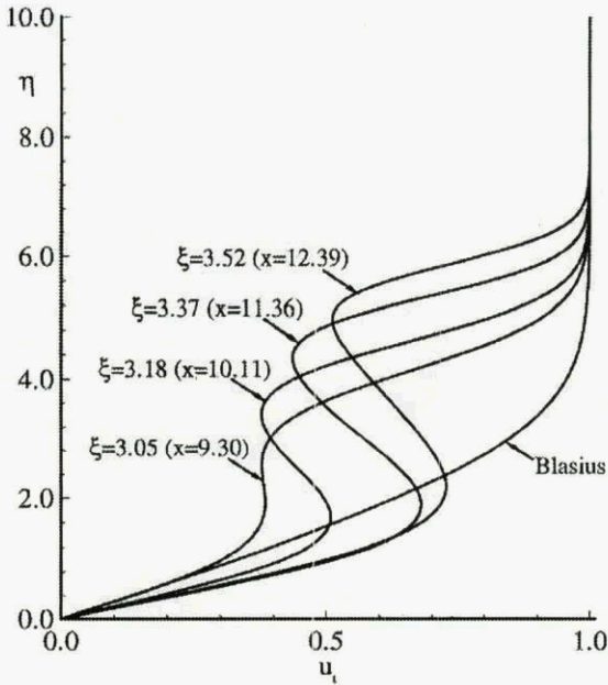
Figure 2. Streamwise evolution of mean profiles of total velocity for constant curvature case.
