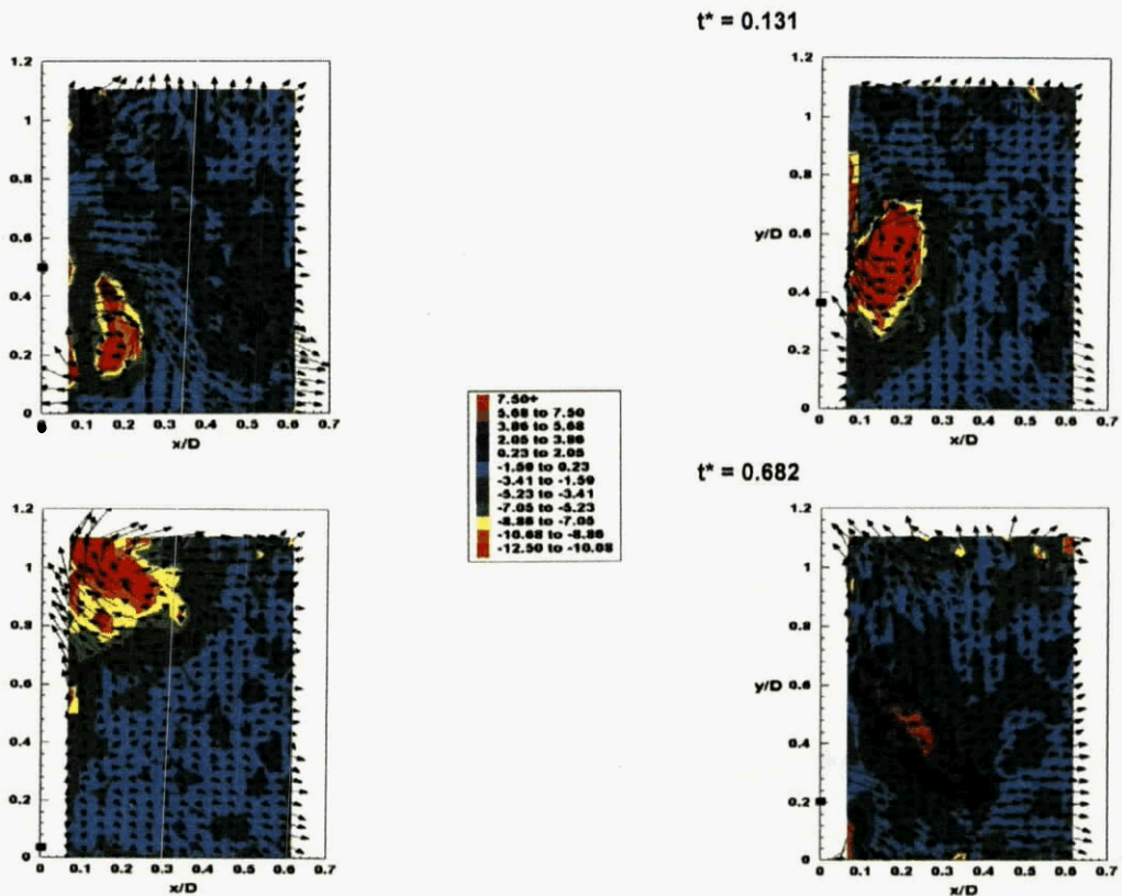
Fig. 17. Vorticity-velocity vector plots in the axial plane for clapping. The velocity perturbations are with respect to freestream velocity. Filled squares on the y -axis indicate the location of flap trailing edge in this and succeeding figures. Note that, when the flap is at outboard extremity, the outer-most vortex trajectory is at 70^\circ to the x -axis which is much larger than the flap trailing edge angle of 30^\circ .
