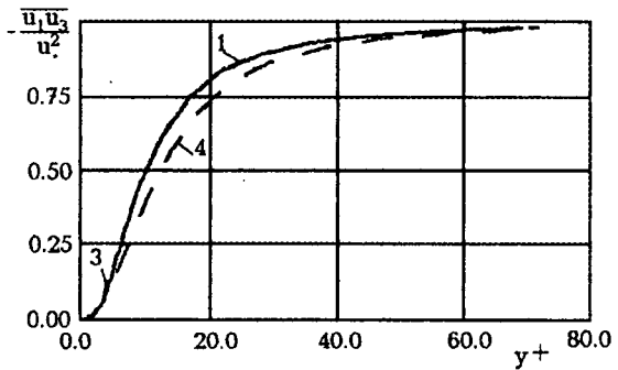
Fig.7. Shear stresses.
