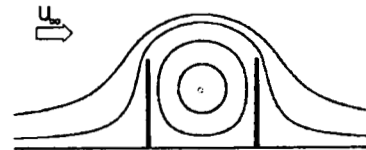
Fig. 12. Flow pattern with the standing vortex in the system two plates
