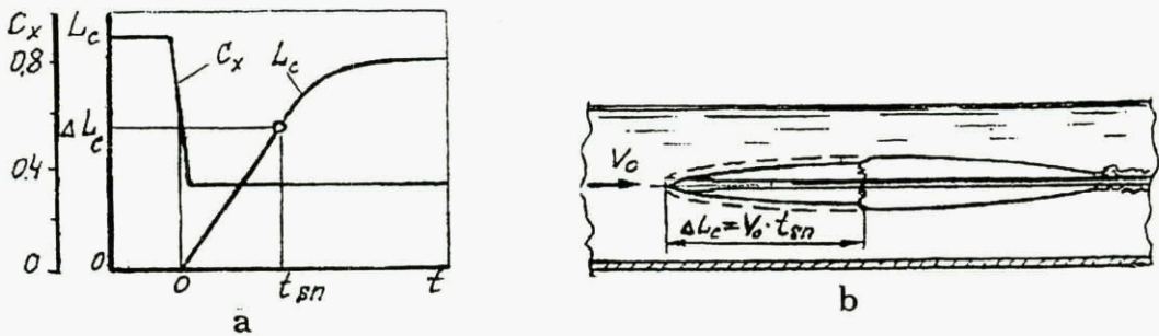
Fig. 11. Scheme of determination of the speed of changing the cavity shape.
