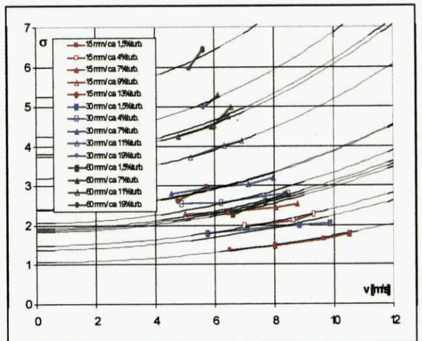
Fig. 7: Cavitation inception at the blunt test body family, in the conventional plot \sigma -value versus flow velocity, for turbulence levels of the free flow from natural up to ca. 20 %
