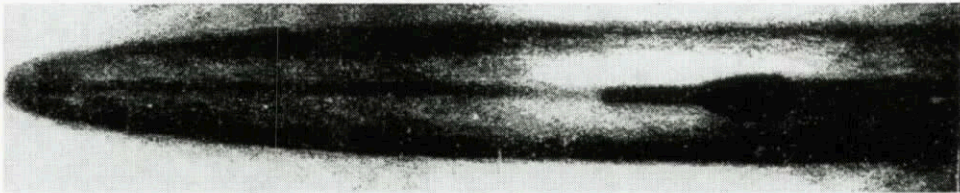
Fig. 8. Supercavity formed by water jet coming from the opposite direction.
