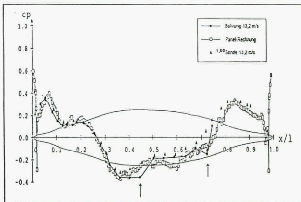
Fig. 6 Pressure distribution, experimental and numerical data.
