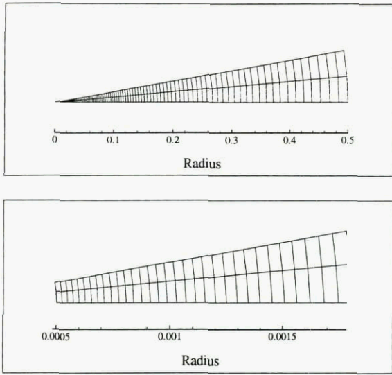
Figure 1 : Bubble mesh
