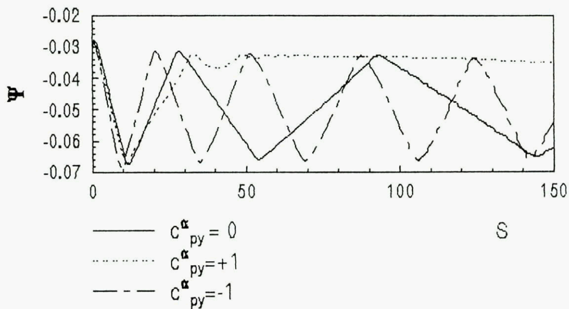
Fig. 9. Influence of C_{py}^\alpha on body motion — dependence of pitch angle on body path
