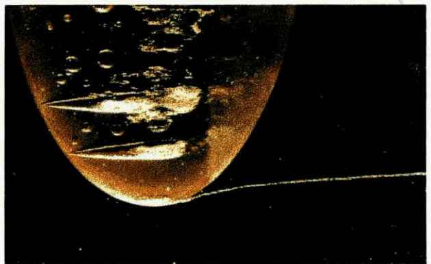
c) Negative tensile strength of the test water; travelling bubble and developed tip vortex cavitation; V_\infty = 9,50 m/s, \sigma = 0,69
