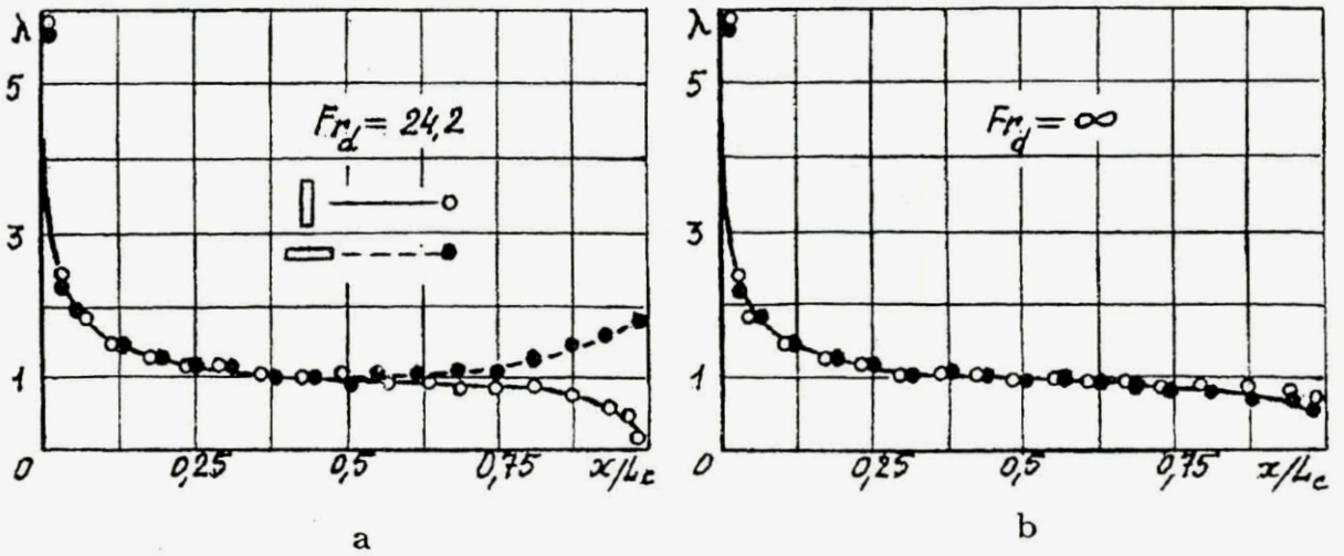
Fig. 16. Changing the section aspect ratio along the length of cavity past a rectangular cavitator with side ratio 1 : 6.
