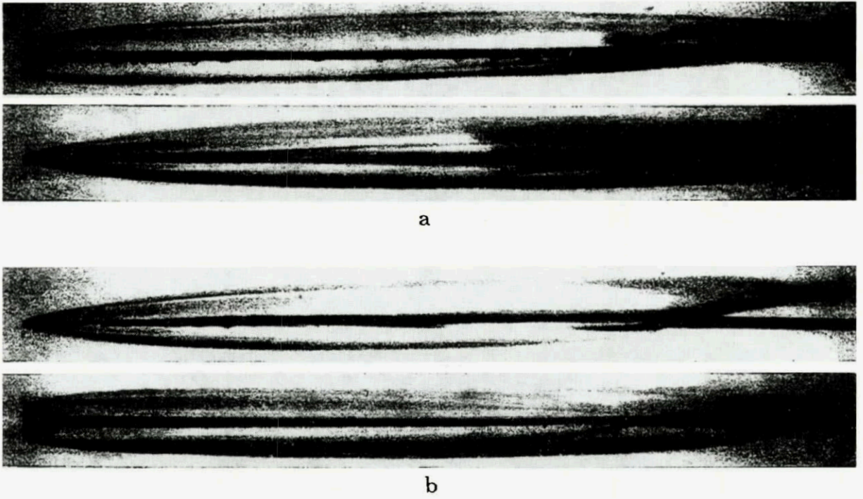
Fig. 15. Photographs of cavities past the rectangular cavitator with side ratio 1 : 6 at \sigma = 0,0364, Fr_d = 24,2 and various orientation of cavitator in the stream.
