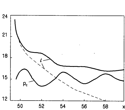
Fig.16. Histories of cavity length and pressure during vertical water penetration at V_0 = 9 m/s (DIVE).
