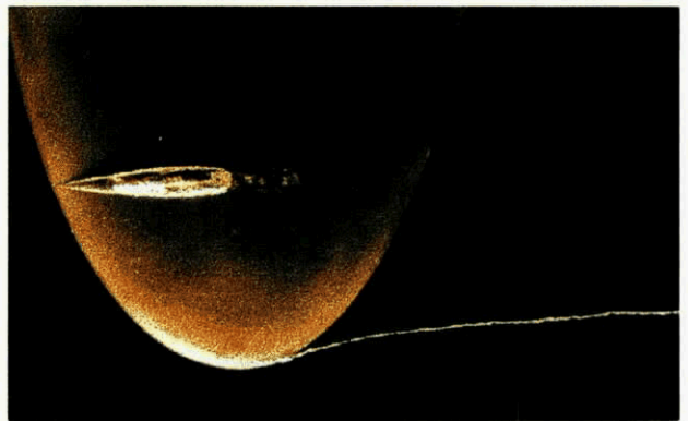
b) Zero tensile strength of the test water; beginning tip vortex cavitation; V_\infty = 9,50 m/s, \sigma = 0,69
