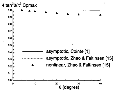
Figure 3: Non-dimensionalized maximum pressure coefficient during water entry of a wedge with constant downward velocity V . Presented as a function of the deadrise angle \theta .
