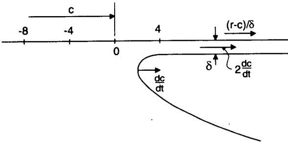
Fig. 3 2-D inner flow domain at the spray root during water entry of blunt axisymmetric body.
