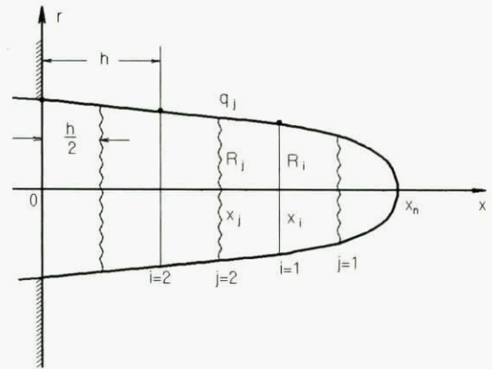
Fig.4. Calculation scheme of water penetration through the rigid wall.
