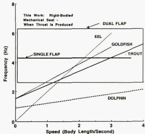
Fig. 4. Comparison of flapping frequencies of the rigid-bodied mechanical seal with those of aquatic animals (refs. 19, 20, 21, and 26). At a given speed, frequency range may be \pm 0.5 Hz.
