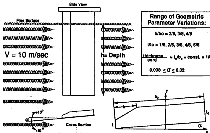
Fig.2. EXPERIMENTAL GEOMETRY
