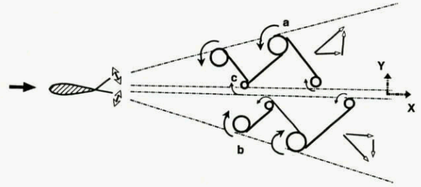
Fig. 28. Schematic of vortex train in waving mode showing the origin of axial and cross-stream force vectors.
