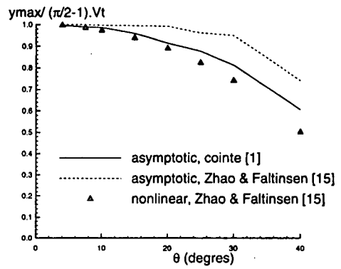
Figure 5: Non-dimensionalized position y_{max} of pressure pic during water entry of a wedge with constant downward velocity V . Presented as a function of the deadrise angle \theta .
