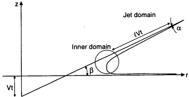
Fig. 4 Attached jet flow during water entry of blunt axisymmetric body.
