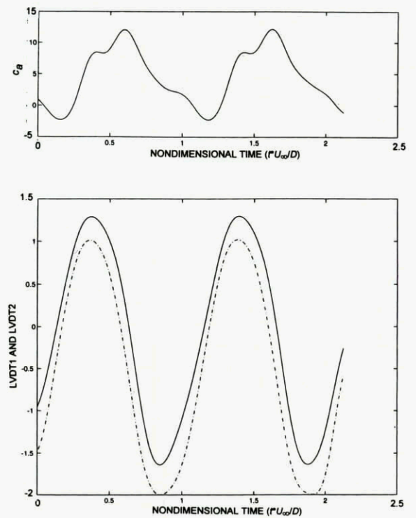
Fig. 10. Ensemble-averaged axial force and flap opening due to dual-flapping foils. High LVDT values = flap fully open; low LVDT values = flap fully closed. The flaps are actually in opposite phase.
