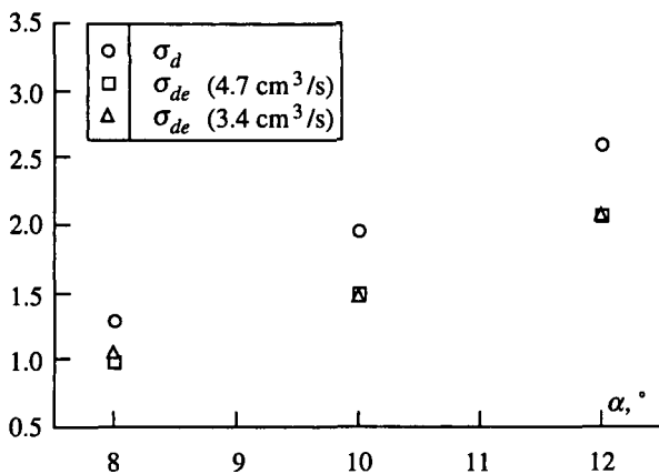
Fig. 3 : Desinent cavitation number as a function of the angle of attack for two injection rates ( Re = 10^6 , polymer concentration : 1000 ppm).
