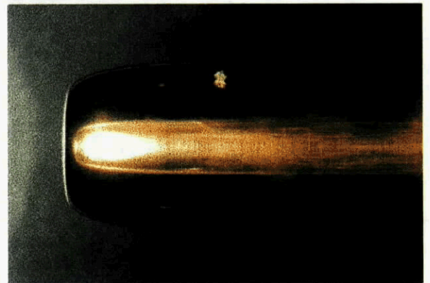
Cavitation inception at \sigma = 0.41 , V_{\infty} = 8.0 m/s
