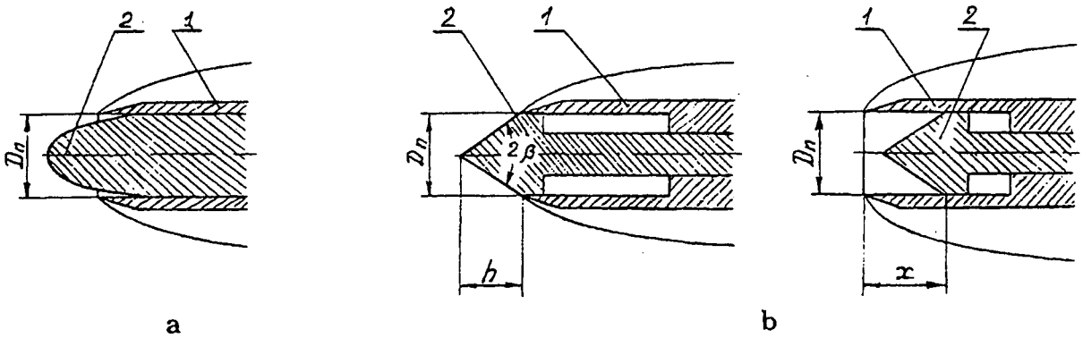
Fig.3. Schemes of cavitators with variable drag.
