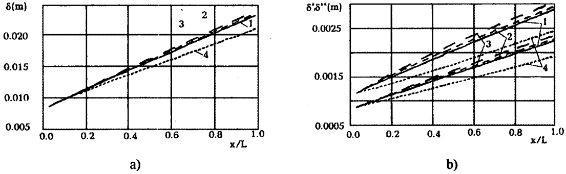
Fig.3. Dimensional value of a) the boundary layer thickness and b) displacement thickness and momentum thickness over:
