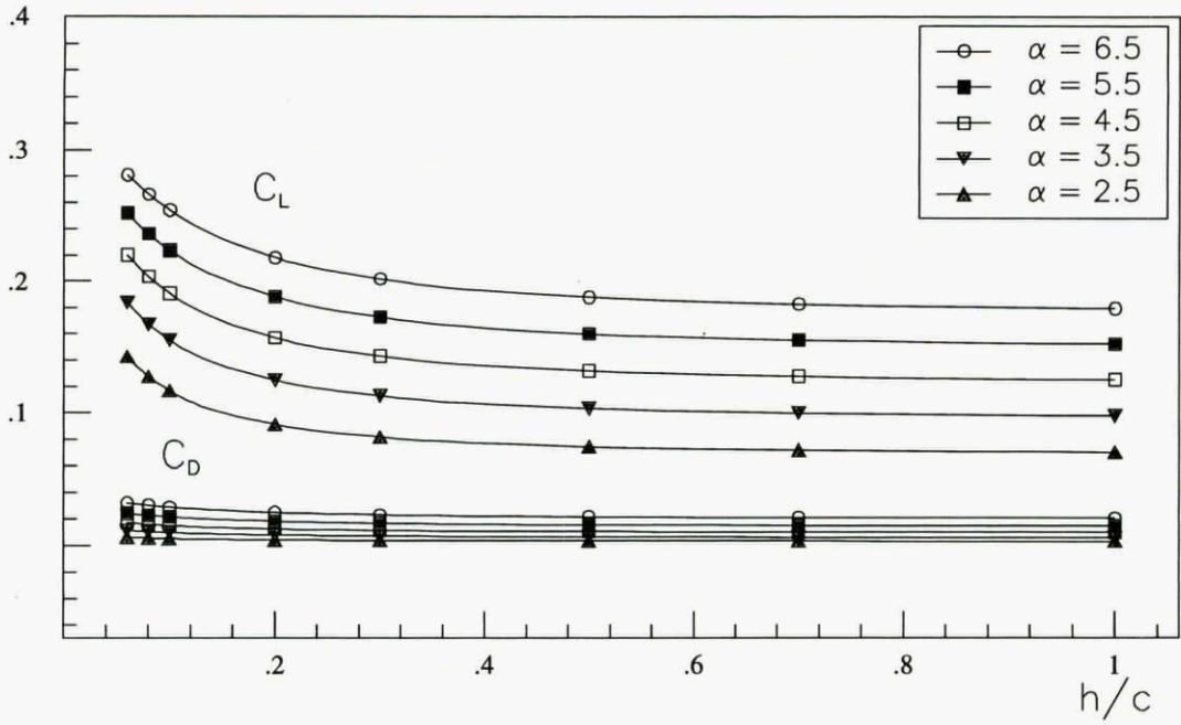
Figure 3: Lift and drag coefficients for a flat plate ( AR=1 ) in steady forward motion ( Fr = 0.5 ): effect of the incidence \alpha and of the distance h/c from the water surface.
