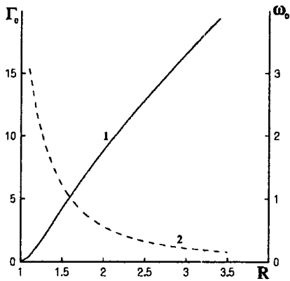
Fig. 4. Dependence of circulation \Gamma_0 (curve 1) and eigenfrequency \omega_0 (curve 2) of standing vortex in the wake of cylinder against its locus
