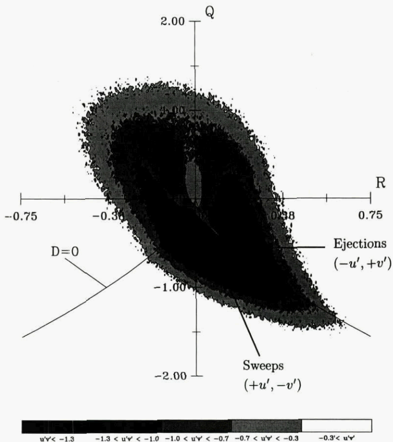
Figure 5: Time-averaged Reynolds shear stress ( -u'v' ) generating events associated with the four incompressible flow topologies. The values of the contour levels shown are normalized by u_\tau^2 (from Chacin et al. [5]).
