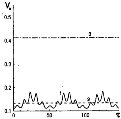
Fig. 8. Velocity of vortex pair vorticity center above a wavy wall in resonant regime
