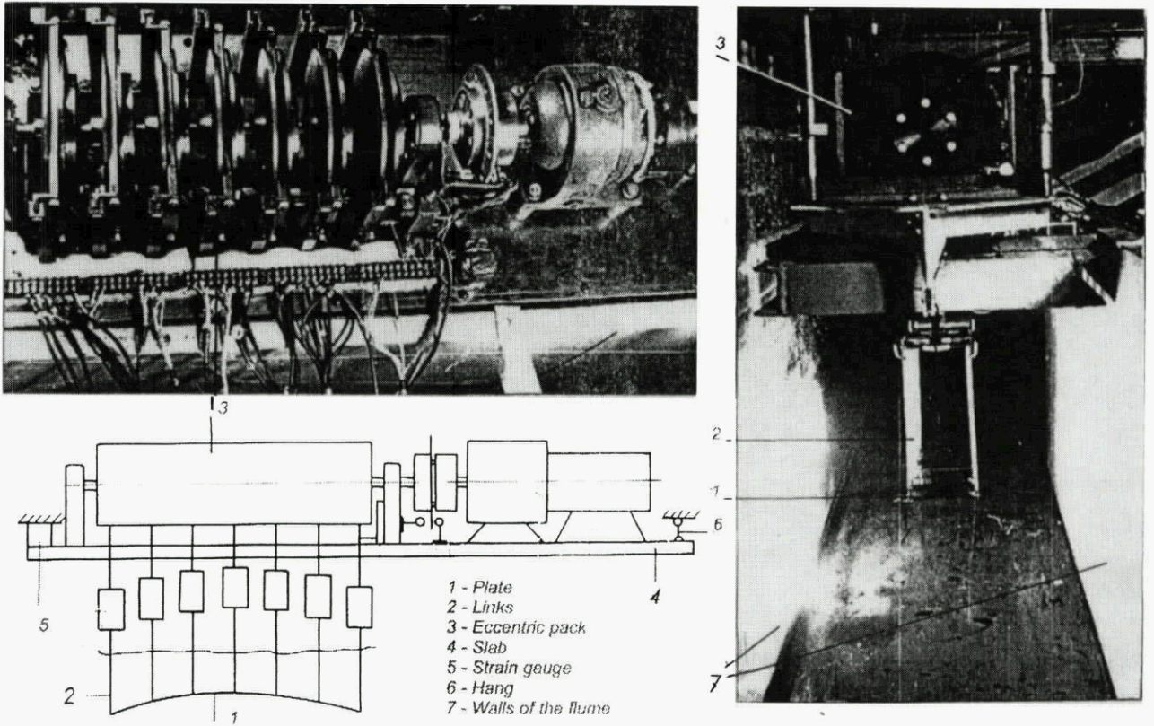
Fig. 1. Experimental installation.
