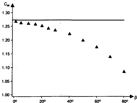
Fig. 9 Wetting factor C_w during water entry of a cone with constant downwards velocity. Presented as a function of deadrise angle \beta . \blacktriangle\blacktriangle\blacktriangle , numerical method; —, asymptotic solution.
