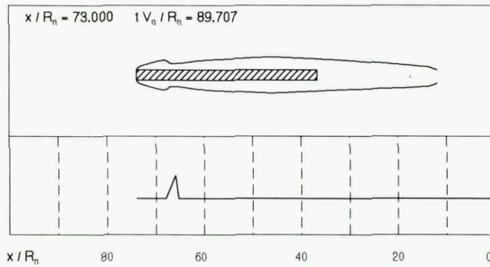
Fig.10. Action of the external pressure perturbation (ENTRY).
