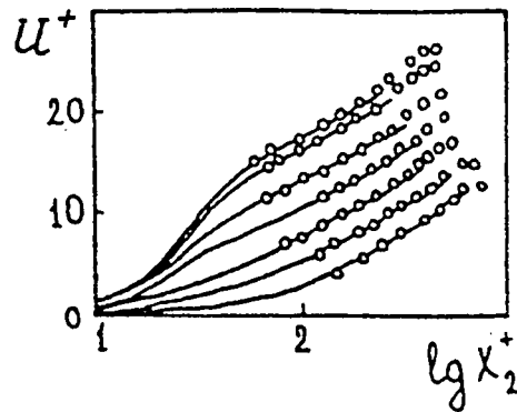
Fig. 1 Comparison of approximate-analytical prediction (line) of velocity profile on rough surface (line) and experimental data of M.D. Millionschikov [1] for pipes with different technical roughness (circles).
