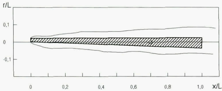
Fig.9. Action of the model angular oscillation (STABILITY).
