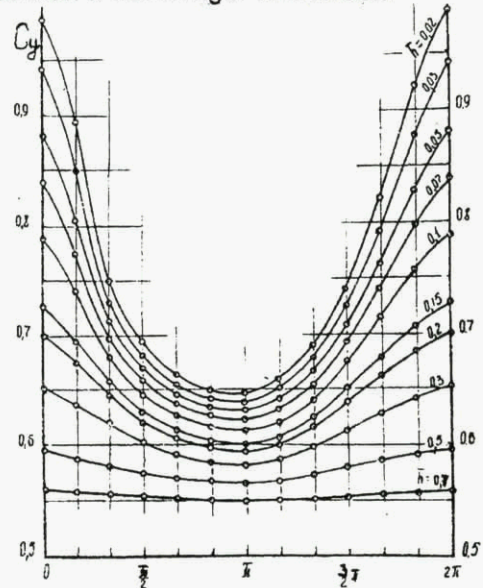
Fig. 5 5.2 All curves, obtained in experiment, of instantaneous significances of lift in a dimensionless kind were subjected to a Fourier analysis with selection average for period of significance of a lift coefficient and coefficients for first six harmonic of Fourier serieses
