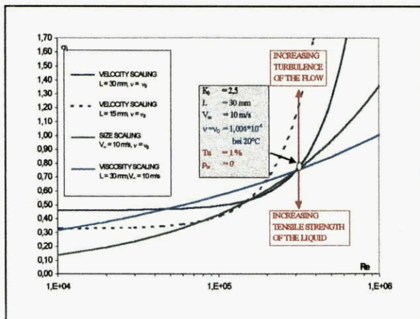
Fig. 10: Variations of \sigma_1 with Reynolds number, by changing V_\infty , L and \nu separately.
