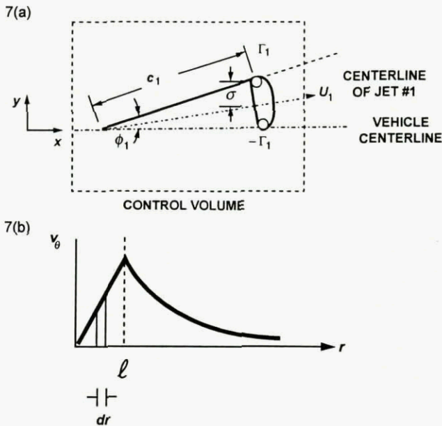
Fig. 7. Vortex doublet (a) and cross-sectional distribution of azimuthal velocity in the shed vortices (b).
