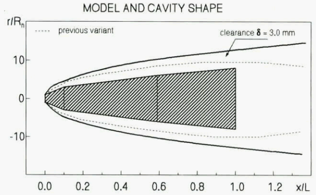
Fig.2. Computation of the cavity shape (SUPERCAVITY).
