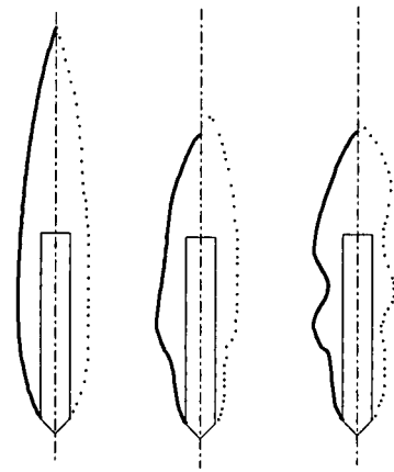
Fig.17. Comparison of computed and experimental cavity shape at V_0 = 9 m/s (DIVE).
