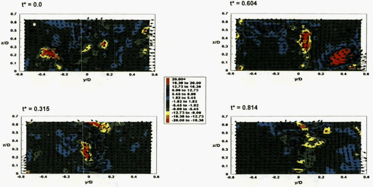
Fig. 20. Vorticity-velocity vector maps in the cross-stream plane in the waving mode; x/D = 0.066 . Filled square markers at z/D = 0.5 within each frame indicates flap location.
