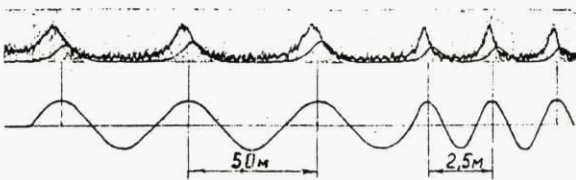
Fig. 4 On Fig. 4 the typical fragments of an oscillogram of a continuous entry in time of lift originating on a wing, driven on small
