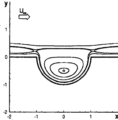
Fig. 3. Phase portrait of vortex trajectories in a cavity
