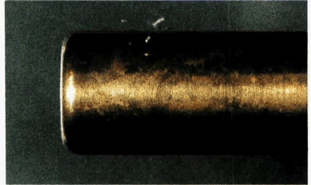
a) cavitation inception, S = 0.08 m/s (Tu = 1%), \sigma = 1.78 , V_\infty = 8.0 m/s, L = 30 mm
