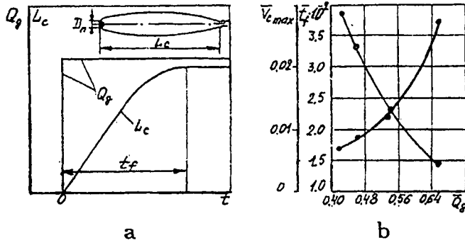
Fig. 1. Graph of the cavity length increase after the supply beginning (a) and dependence of the length increase speed \bar{V}_{c_{max}} and the cavity formation period t_f on the gas supply value.
