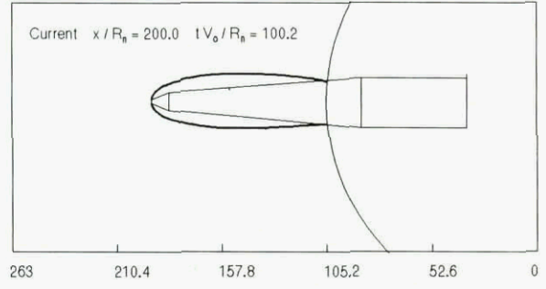
Fig.8. Computer simulation of water penetration from within the gas bubble (ENTRY).
