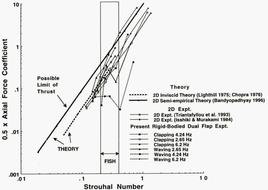
Fig. 12. Comparison of measurements of axial force (thrust) coefficient.
