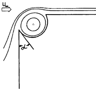
Fig. 9. Flow pattern near bend of the boundary with vortex chamber
