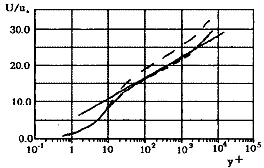
Fig.5. Velocity profiles.
