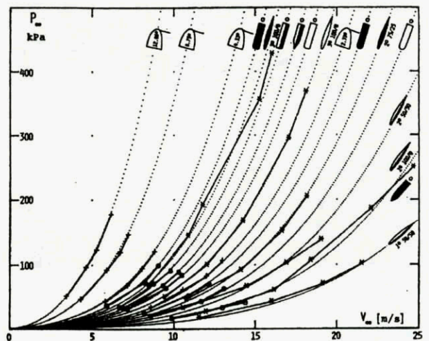
Fig. 4: Pressure - velocity relation for cav. inception for all body types in liquids of zero tensile strength
