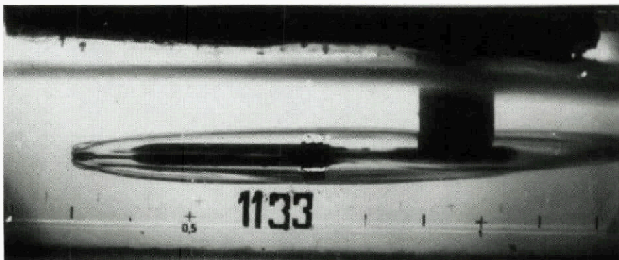
Fig. 6. Cavity behind star - shaped cavitator.
