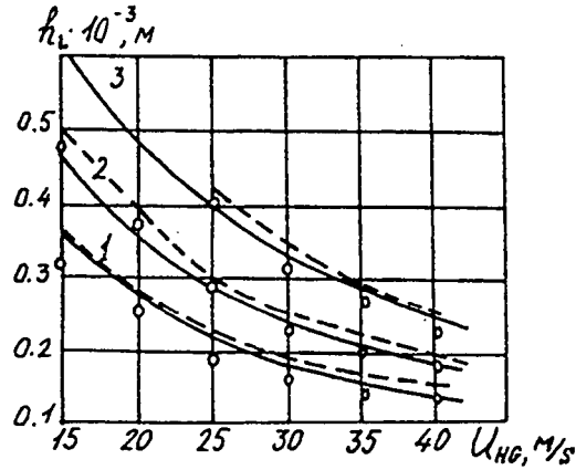
Fig. 7. Comparison of liquid film thickness h_L computation (lines) and O.A., Povarov, G.A., Phillipov, E.A., Vasylychenko experimental data [10] (circles), where: 1 - Re_L = 100 ; 2 - Re_L = 200 ; 3 - Re_L = 400 ; dash line - numerical method of calculations [8]; continuous line - integral method of predictions [7].
