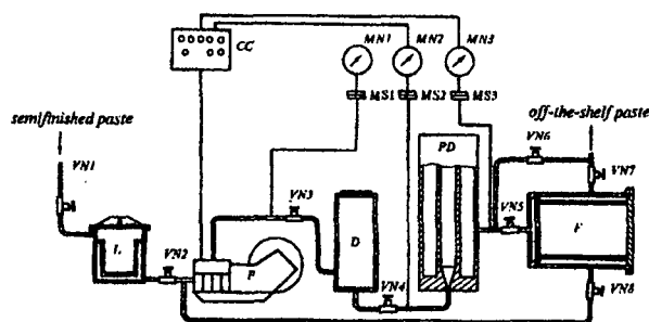
Fig. 7 Schematic of the hydrodynamic cavitation plant for dispersing the pastes of aqueous – dispersion paints: VN1 - VN8 – valves; L - trap; P - pump; CC - 6control cabinet; MN1 - MN3 – manometers; MS1 - MS3 - membrane separator; PD - powder dispenser; F - filter; D - damper.
