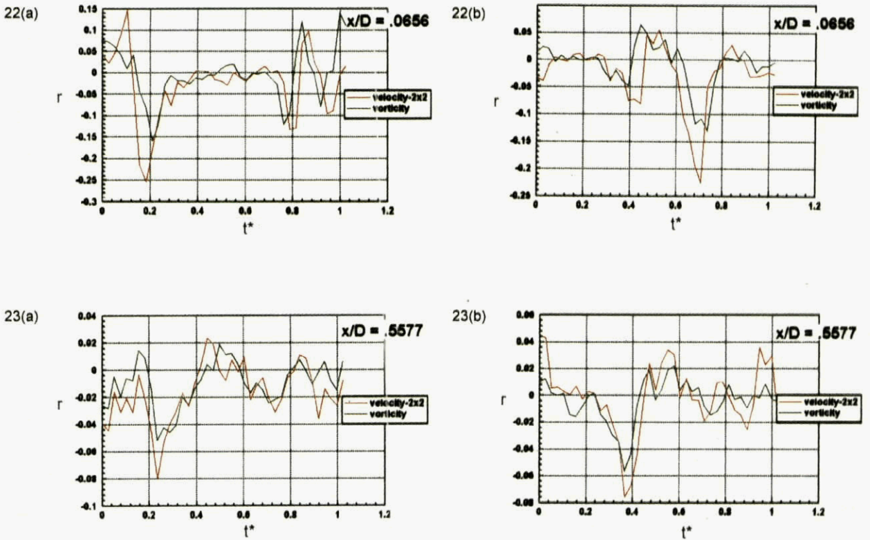
Fig. 23. Circulation distribution at a downstream station ( x/D = 0.5577 ) compared to that in Fig. 22, (a) waving and (b) clapping
