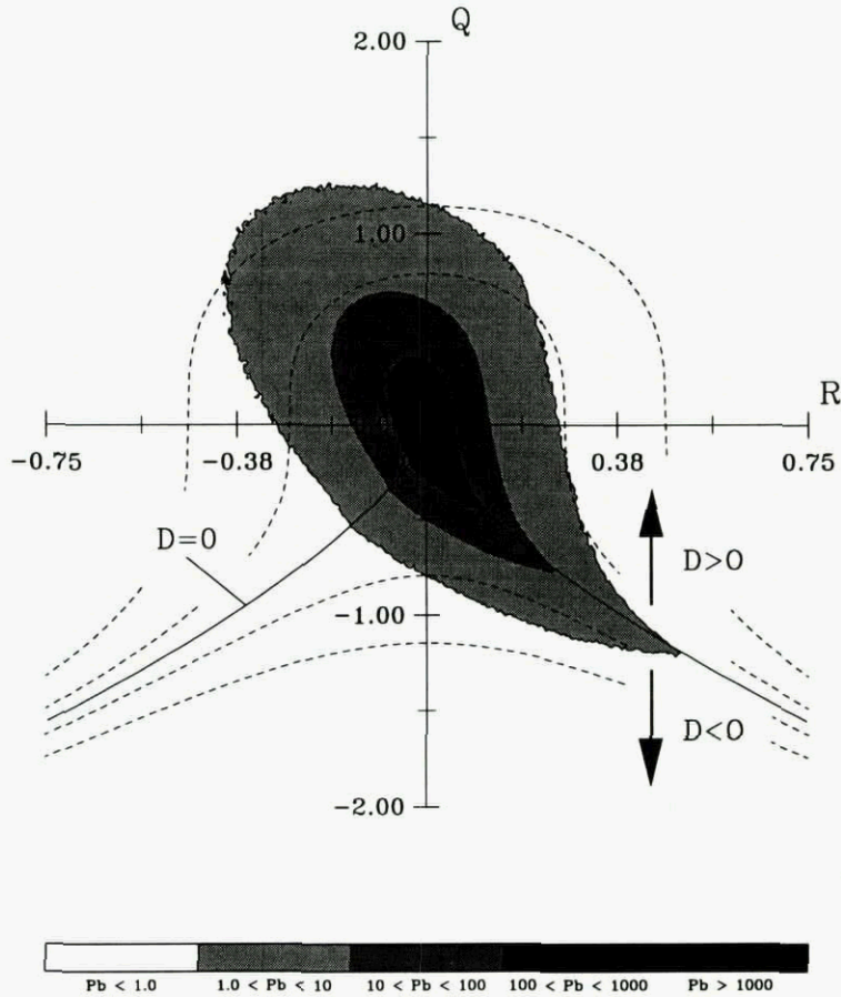
Figure 2: Contour plot of joint probability distributions of the invariants of the velocity gradient tensor at Re_\theta = 670 (from Chacin et al. [5]).
