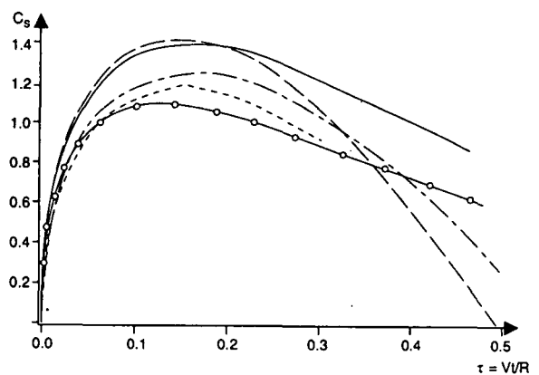
Fig. 12 Slamming coefficient C_s during water entry of sphere with constant downwards velocity V versus dimensionless time. \circ - \circ - \circ , numerical method and pressure integration; —, numerical method and VdA_{33}/dt ; ----, Eq. (23) (Miloh [26]); - · - · -, Eq. (24) (Miloh [26]); - - - - -, experiments (Moghisi and Squire [27]).
