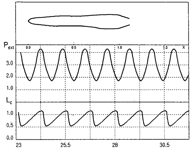
Fig.12. Computer simulation of the ventilated cavity self-induced oscillations (PULSE).
