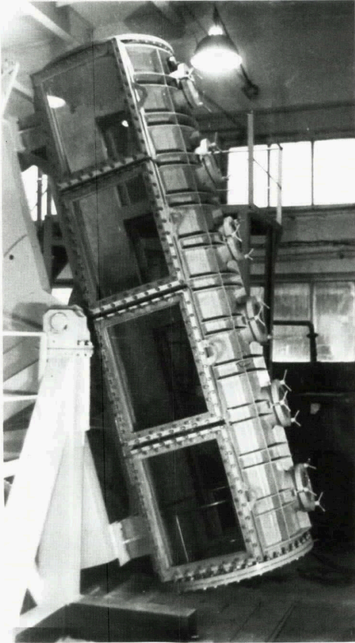
Fig. 1. Stand with varying tank inclination.
