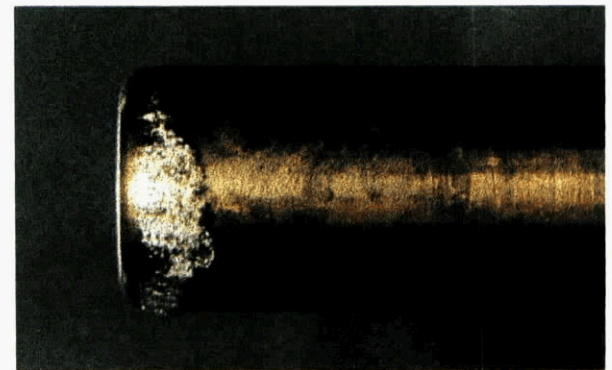
c) fully developed cavitation, S = 0.96 m/s (Tu = 12%), \sigma = 1.78 , V_\infty = 8.0 m/s, L = 30 mm
