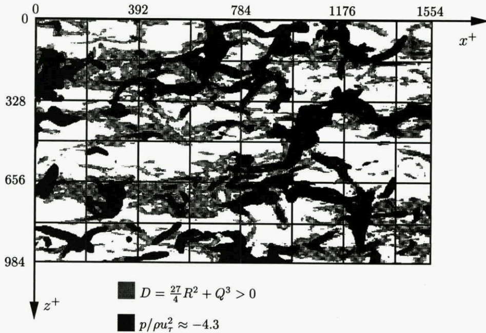
Figure 8: Top view of the computational domain showing regions of positive discriminant (light gray) and isocontours of instantaneous pressure (dark gray). The pressure threshold level is p/\rho u_\tau^2 \approx -4.3 .
