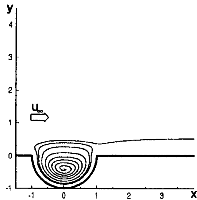
Fig. 6. Trajectory of the standing vortex behind a cavity at flow resonant perturbations
