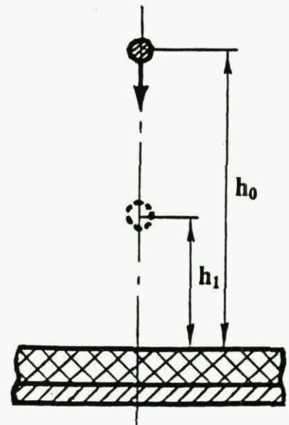
Fig. 3 Measurement of damping properties; damping coefficient depending on the excitation energy, K(P) and loss angles \text{tg } \varphi .
