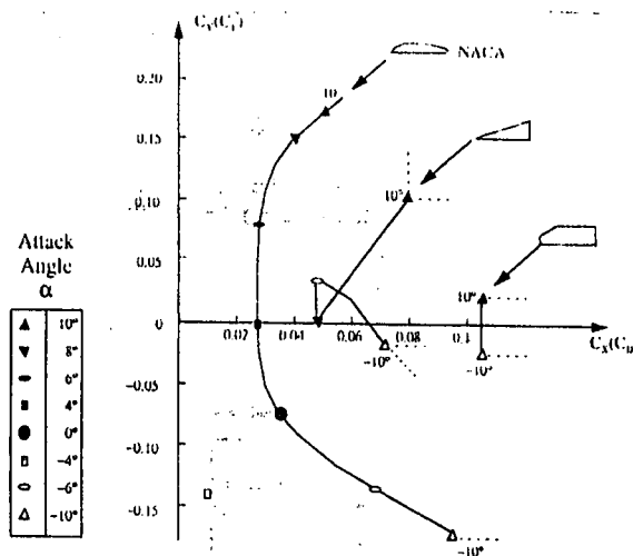
Fig.3. LIFT-TO-DRAG CHARACTERISTICS
