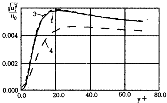
Fig.6. Turbulence energy components.
