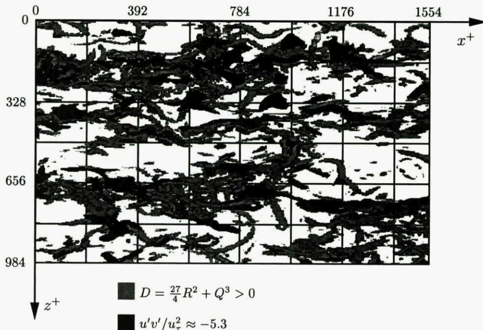
Figure 4: Top view of the computational domain showing regions of positive discriminant (light gray) and isocontours of instantaneous -u'v' (dark gray).
