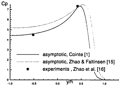
Figure 8: Coefficient pressure, along a wedge with deadrise angle \theta = 30^\circ , immersed at h at the beginning of the impact ( t=0.00435s ).
