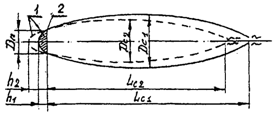
Fig. 2. Scheme of control of the cavity parameters by changing the cavitator drag.
