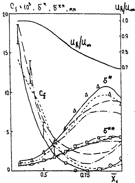
Fig. 4. Comparison of computation (continuous line) and Scottorn - Power' experimental data on two-dimensional boundary layer with rough surface [5] ( \odot, \square, \Delta ). Nomenclature is the same as in Fig. 3., except dash lines - predictions of different researches: - - - T. Cebeci, K.C. Chang [5]; - - - G.F. Sivykh [12]; - - - F.A. Dvorak [13].
