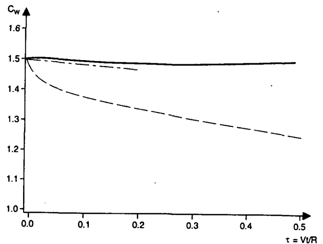
Fig. 11 Wetting factor C_w during water entry of a sphere with constant downwards velocity V versus dimensionless time. —, numerical method; - - -, experiments (Cooper [29]); - · - · -, experiments (Shiffman and Spencer [23]).
