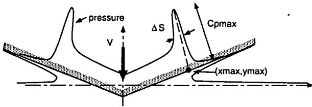
Figure 2: Characteristic parameters describing the pressure distribution.
