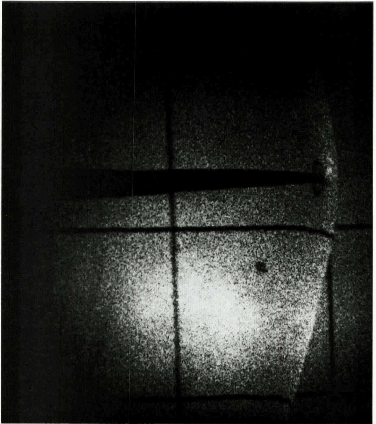
Figure 1 Back-Lit image of a projectile launched at supersonic speeds underwater
