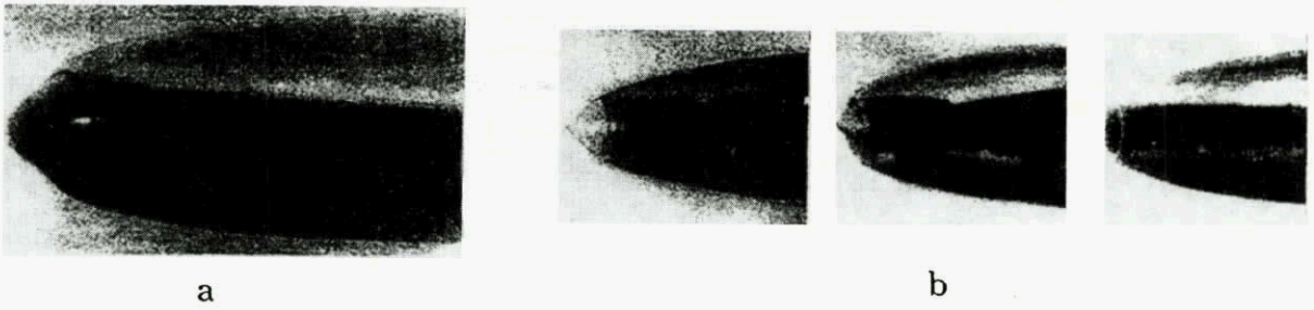
Fig. 5. Photographs of the nose of cavities past cavitators with variable drag.
