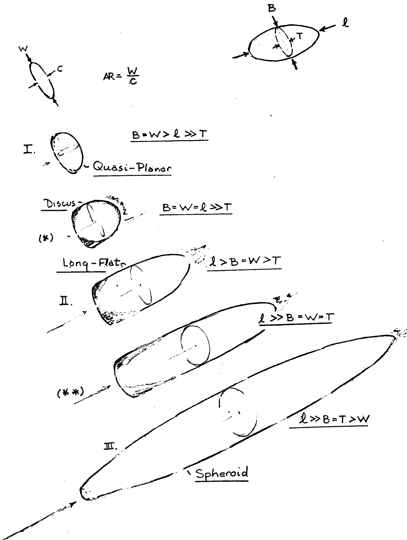
Figure 1: Supercavitating Regimes
