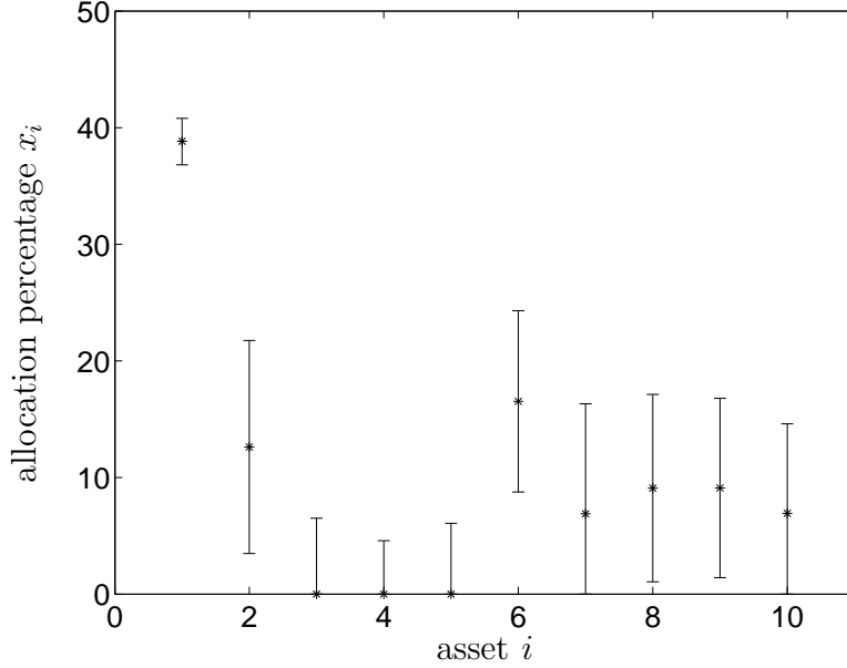
Figure 8: Optimal portfolio allocation (shown as stars) and bounding box (shown as vertical intervals) for the 0.02p^* -suboptimal set.
