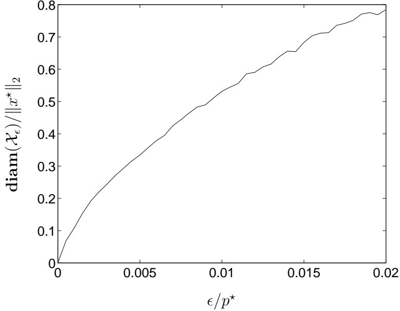
Figure 5: Estimate of normalized diameter of \mathcal{X}_\epsilon versus \epsilon/p^* .
