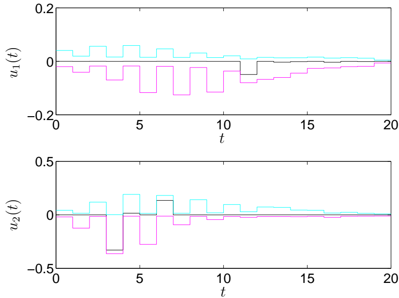
Figure 7: Optimal input, and lower and upper bounds over 5%-suboptimal trajectories.
