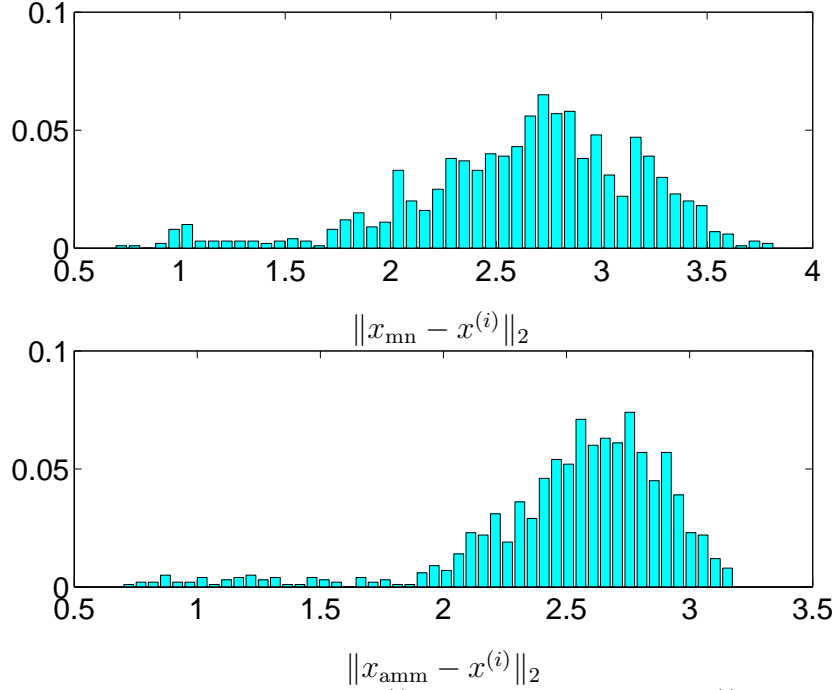
Figure 6: Distributions of \|x_{mn} - x^{(i)}\|_2 (top) and \|x_{amm} - x^{(i)}\|_2 (bottom) over i = 1, \dots, 1000 .
