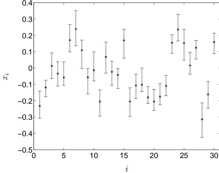
Figure 4: Solution (shown as stars) and bounding box (shown as vertical intervals) of 1%-suboptimal set.
