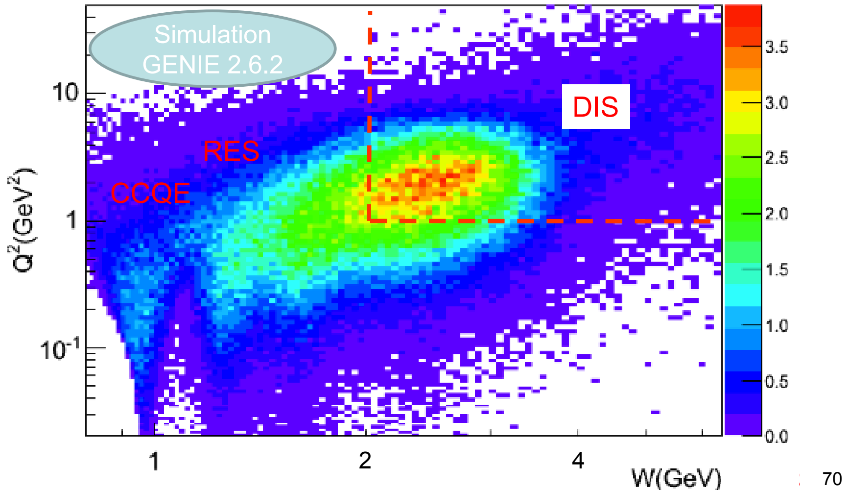
Event statistics for ME neutrino run
