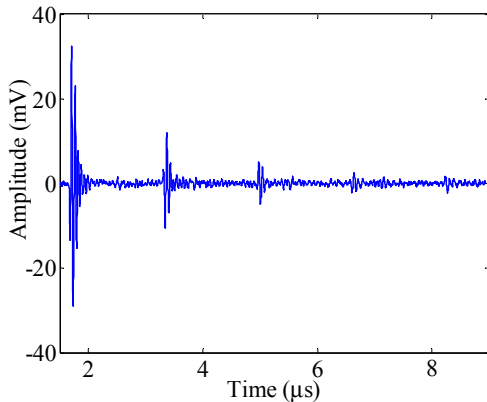
Figure 6. Echo from a Plane Reflector at 1.2 mm
