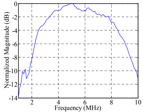
Figure 4. Spectrum of Signal Transmitted from CMUT
