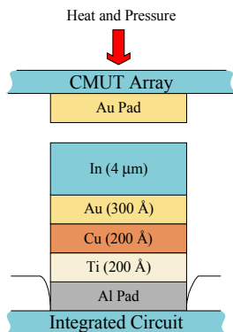
Figure 10. Metal Stack Used for Flip-Chip Bonding
