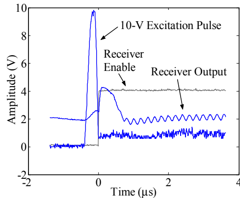
Figure 9. Preamplifier Startup
