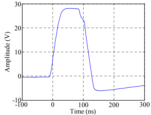
Figure 8. 28-V Transducer Excitation Pulse
