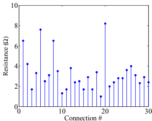
Figure 11. Resistance of Individual Flip-Chip Bond Connections
