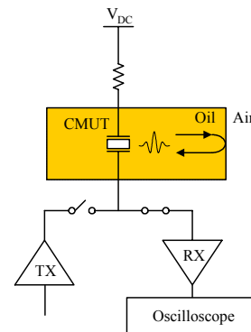
Figure 5. Pulser/Preamplifier Circuit
