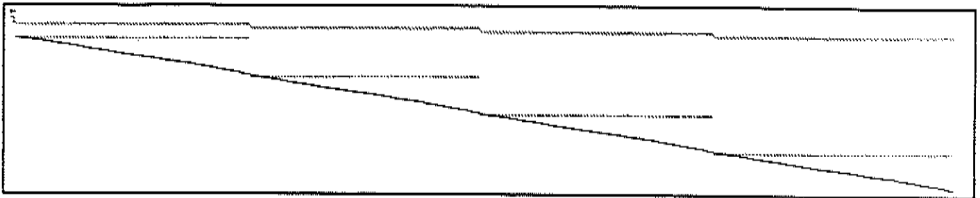
Picture for Problem 39 SHIP04L Magnified 0.25
