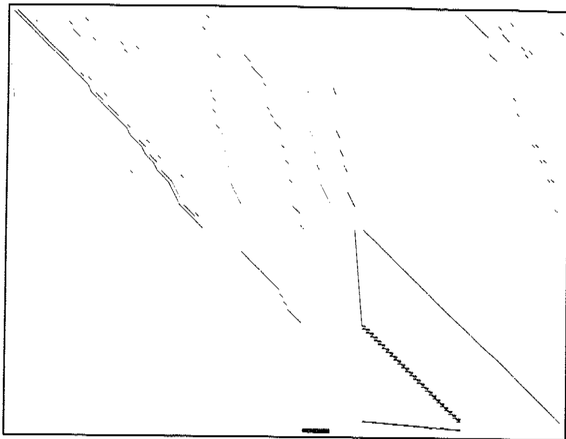
Picture for Problem 35 GANGES Magnified 0.25
