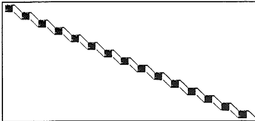
Picture for Problem 32 GROW15 Magnified 0.5
