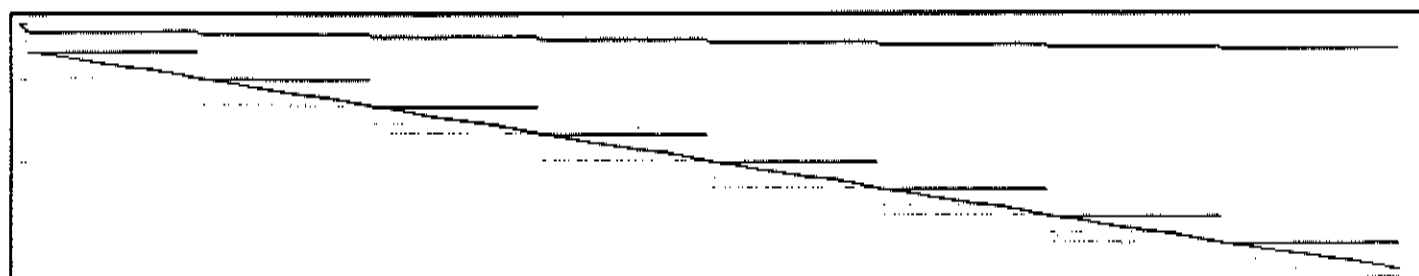
Picture for Problem 50 SHIP08L Magnified 0.125
