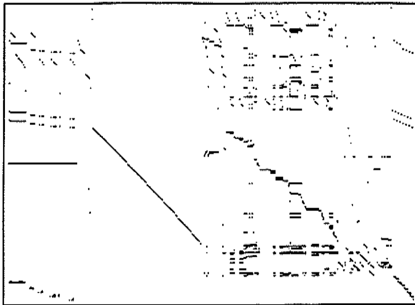
Picture for Problem 9 BORE3D Magnified 1.0
