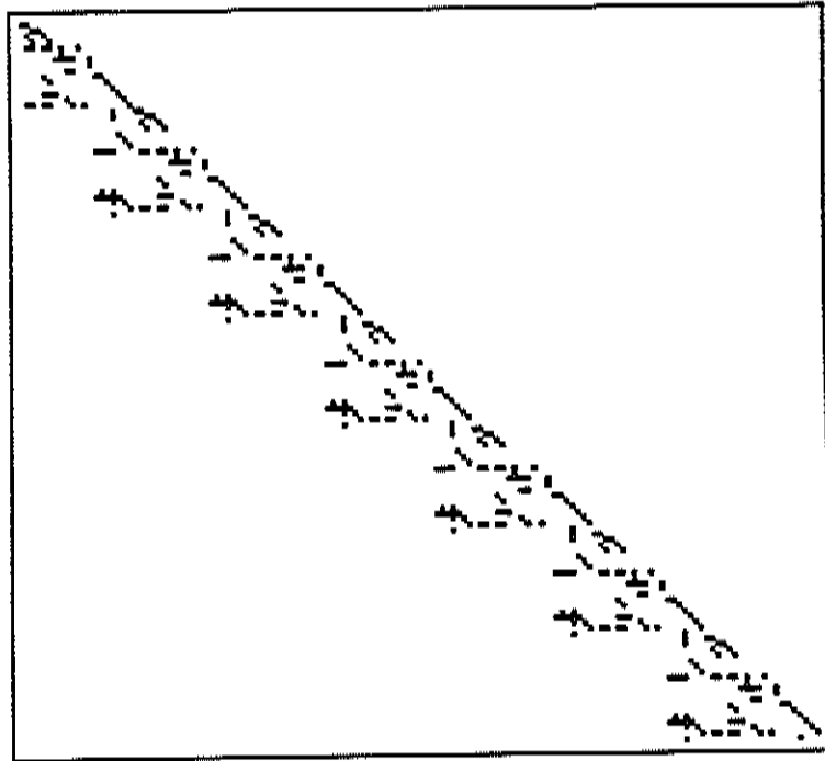
Picture for Problem 4 SCAGR7 Magnified 2.0
