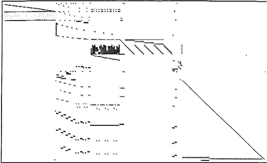
Picture for Problem 34 FFFF800 Magnified 0.5
