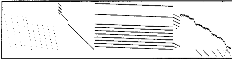
Picture for Problem 47 NESM Magnified 0.125
