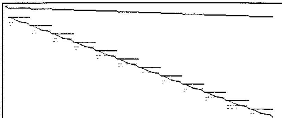
Picture for Problem 44 SHIP12S Magnified 0.125
