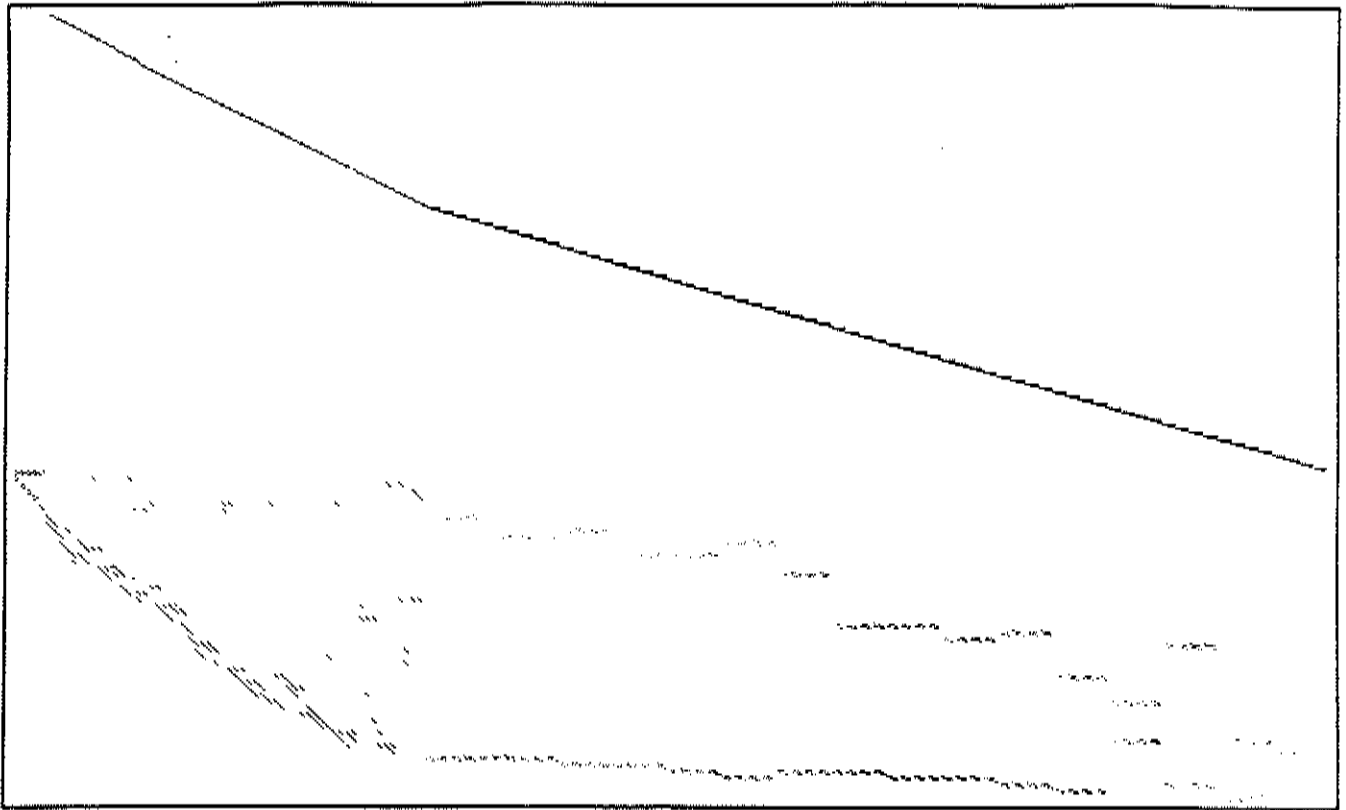
Picture for Problem 41 SIERRA Magnified 0.25
