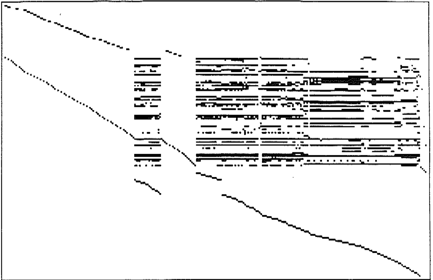
Picture for Problem 24 BEACONFD Magnified 2.0
