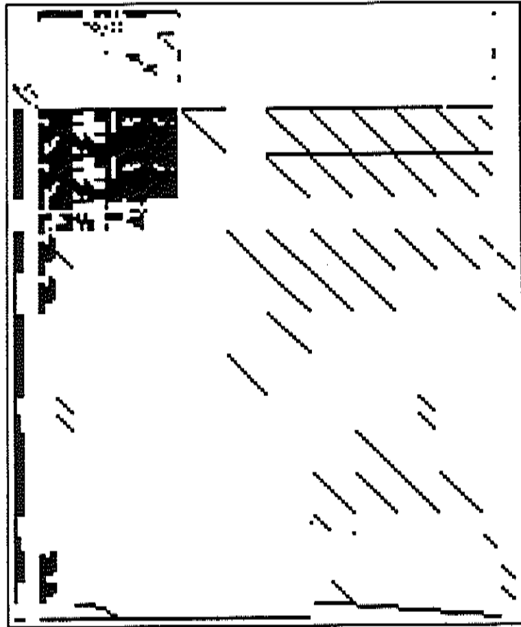
Picture for Problem 15 ISRAEL Magnified 2.0
