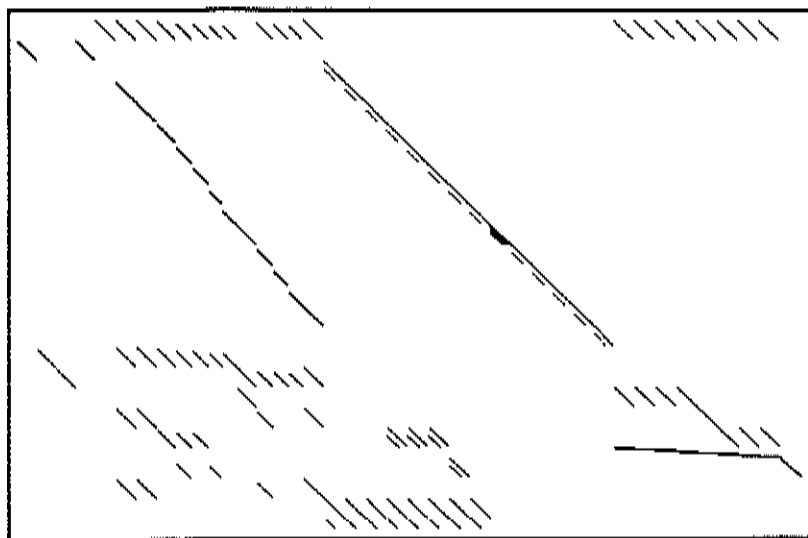
Picture for Problem 16 ETAMACRO Magnified 0.5
