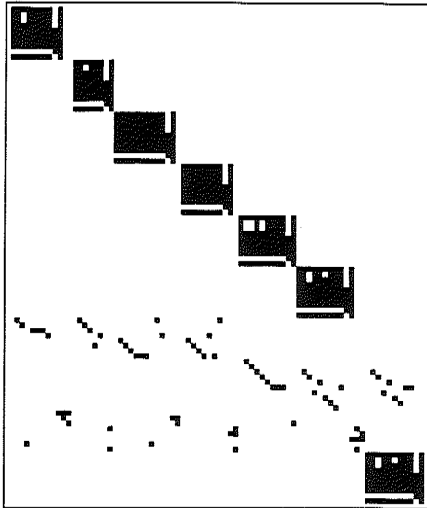
Picture for Problem 5 SHARE2B Magnified 4.0
