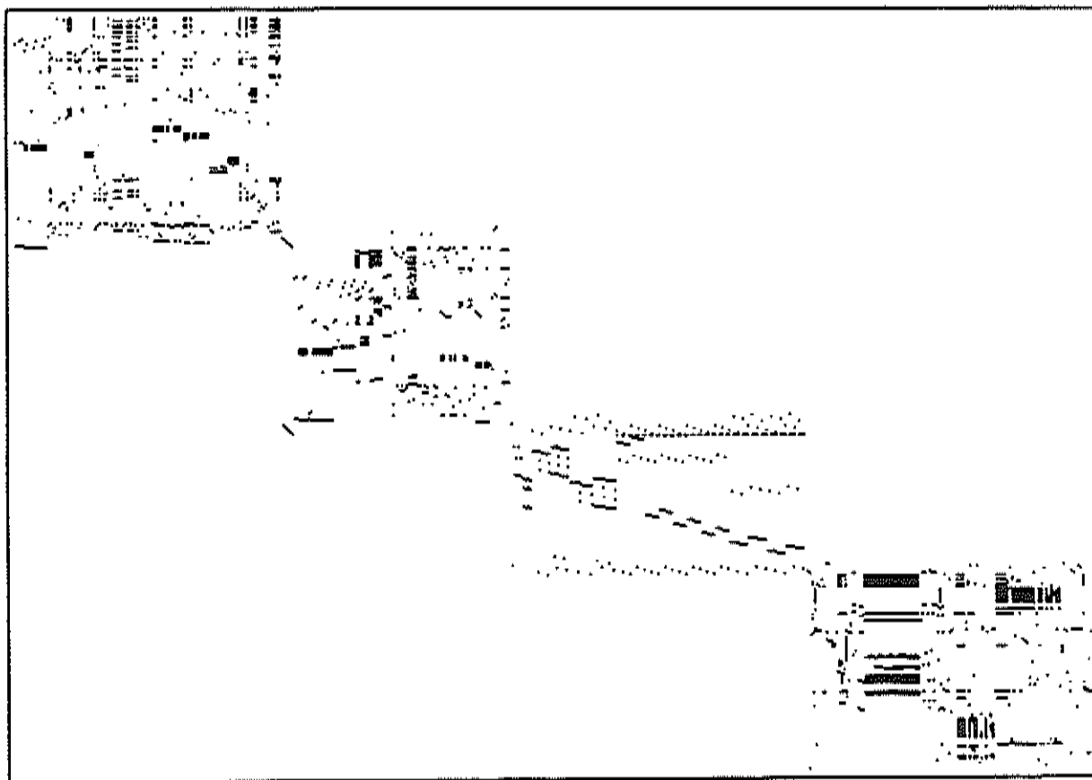
Picture for Problem 17 SCFXM1 Magnified 1.0
