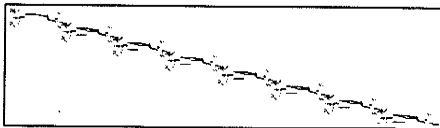
Picture for Problem 40 PILOTWE Magnified 0.125
