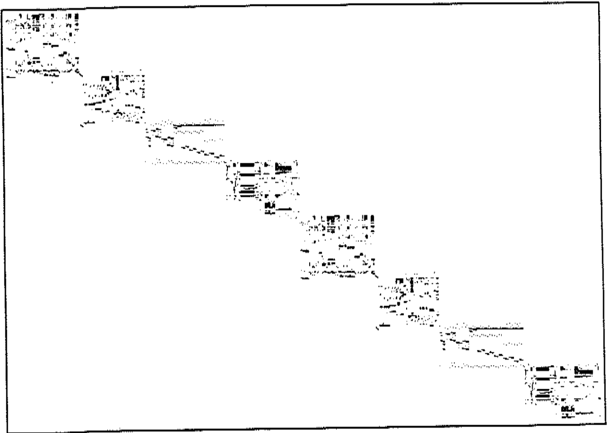
Picture for Problem 30 SCFXM2 Magnified 0.5
