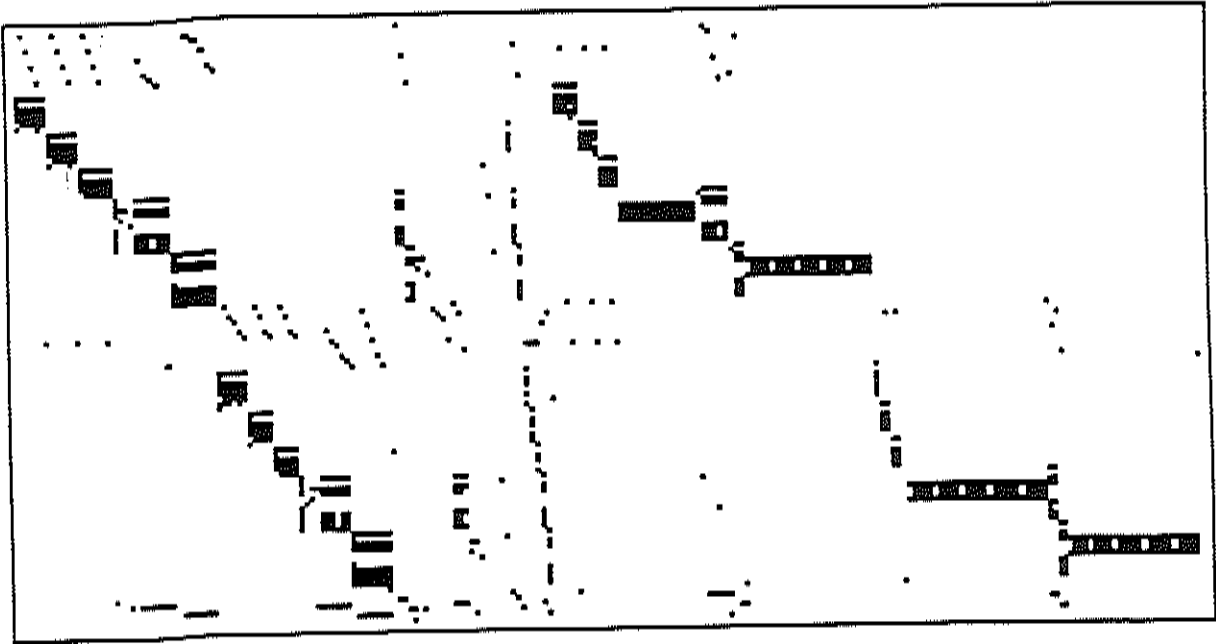
Picture for Problem 8 SHARE1B Magnified 2.0
