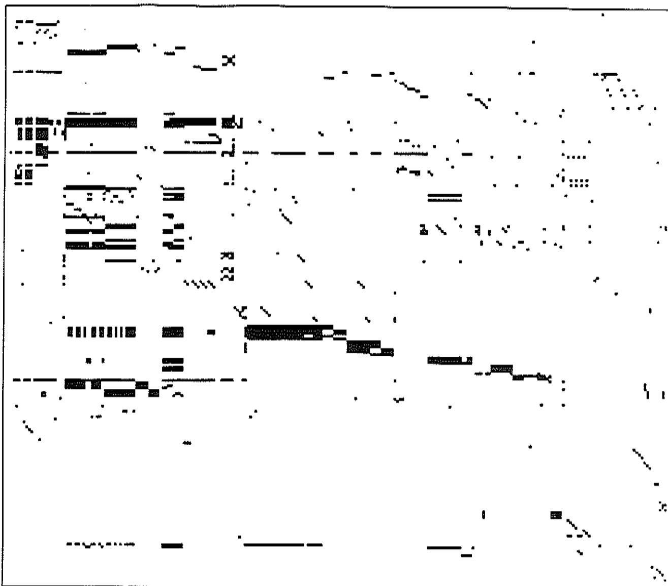
Picture for Problem 14 BRANDY Magnified 2.0
