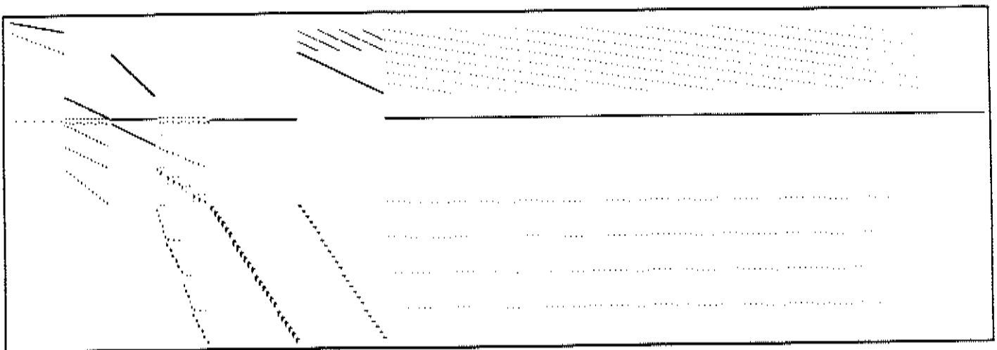
Picture for Problem 21 STANDATA Magnified 0.5
