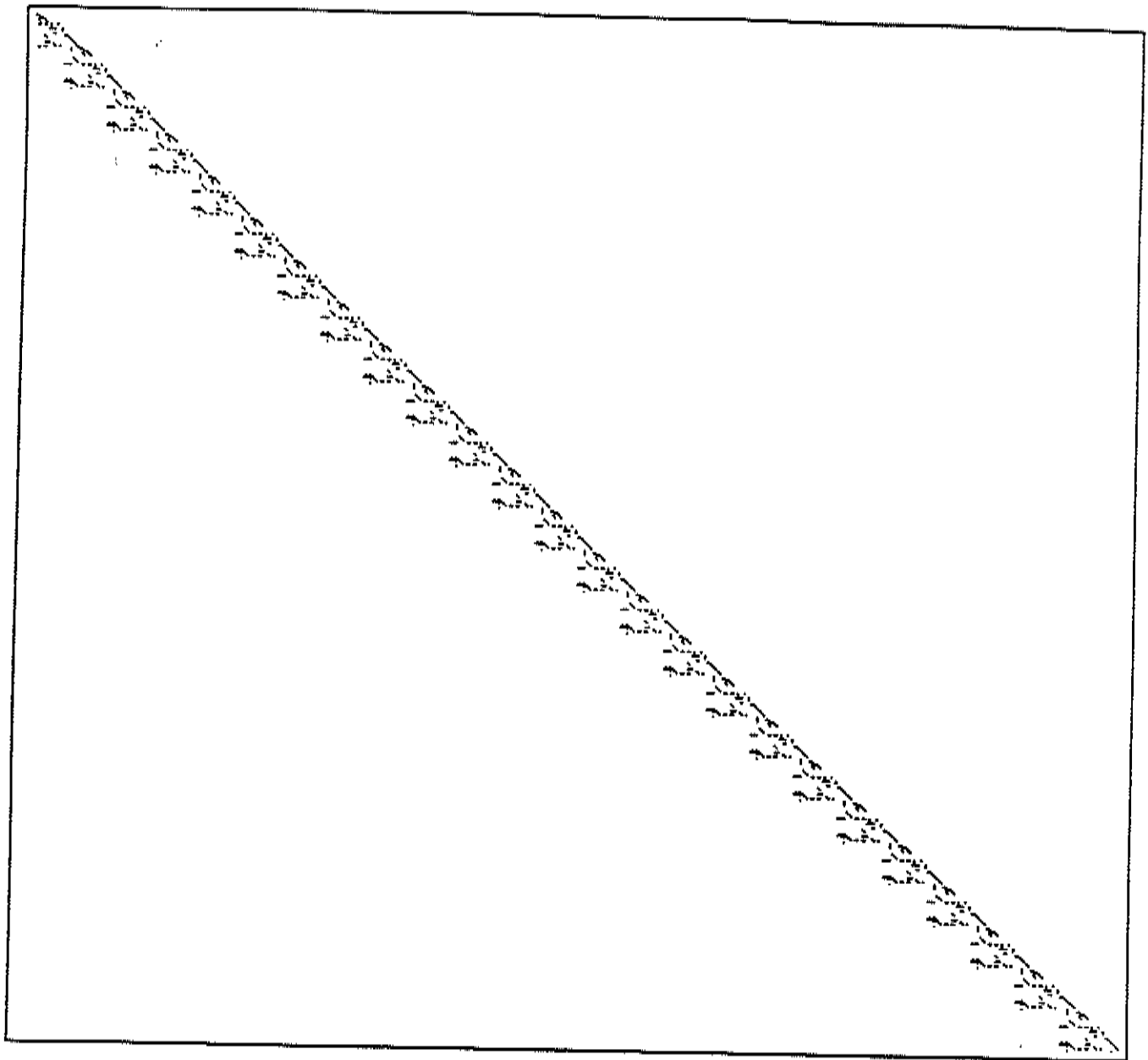
Picture for Problem 12 SCAGR25 Magnified 1.0
