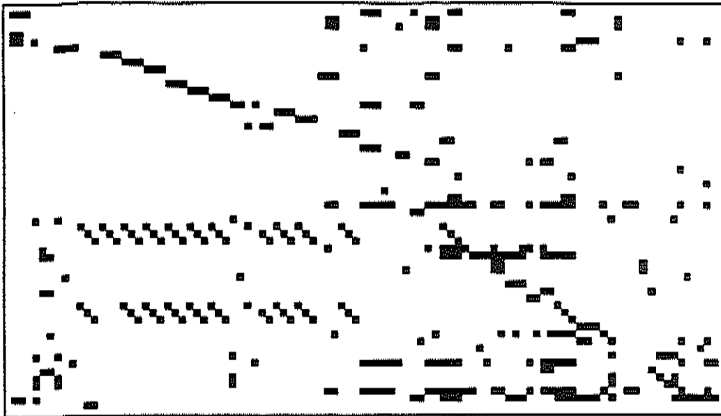
Picture for Problem 2 ADLITTLE Magnified 4.0
