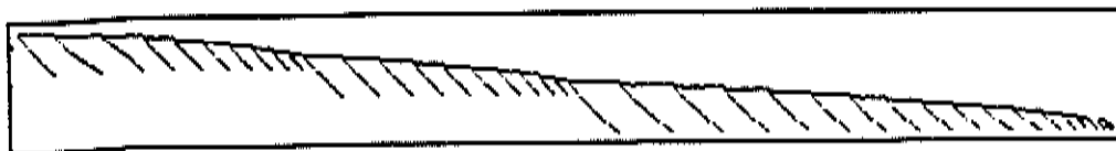
Picture for Problem 22 SCSD1 Magnified 0.5
