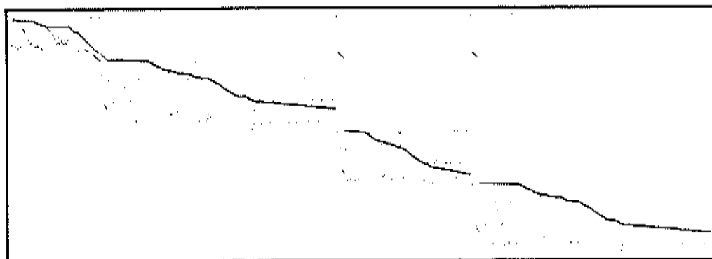
Picture for Problem 28 SHELL Magnified 0.25
