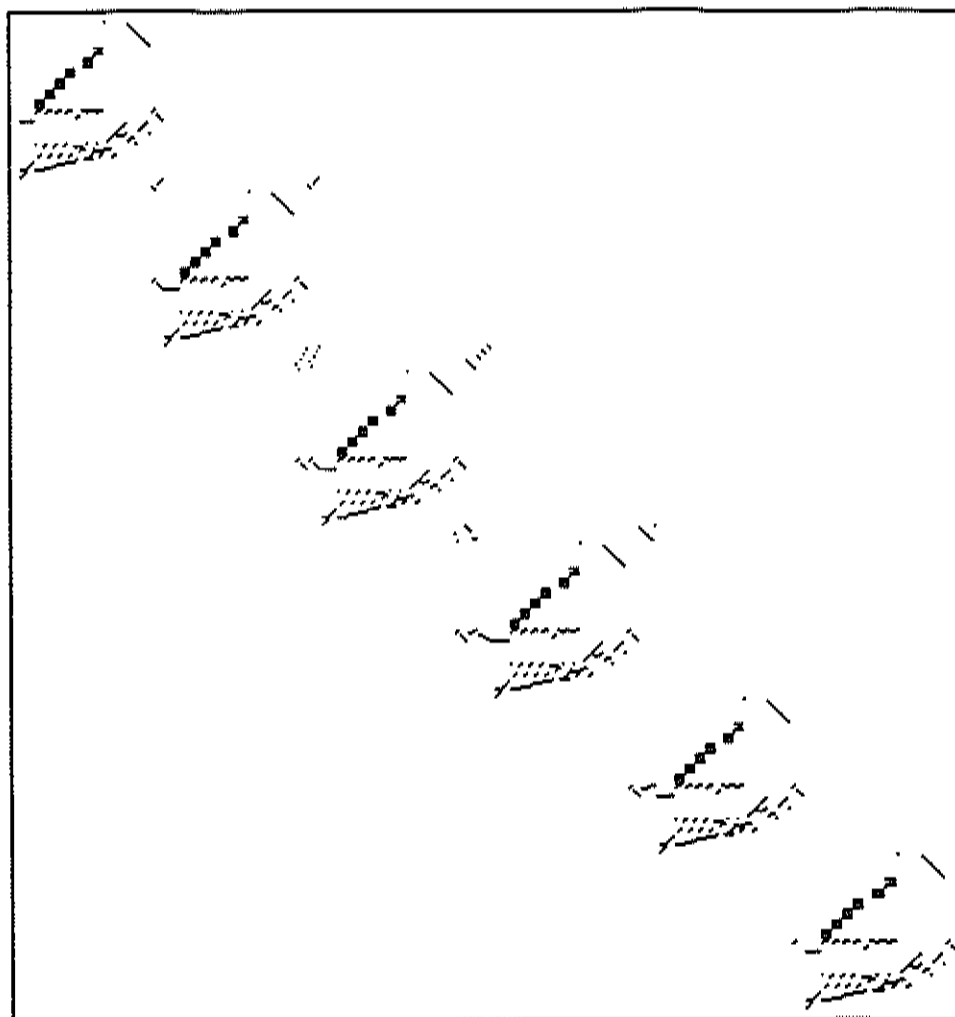
Picture for Problem 10 SCORPION Magnified 1.0
