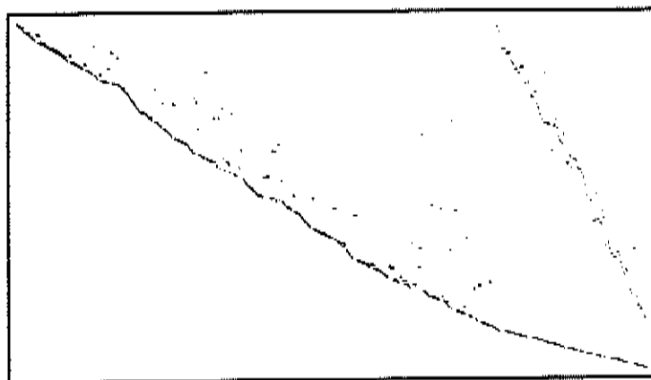
Picture for Problem 23 GFRDPNC Magnified 0.25
