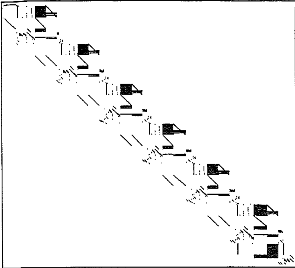
Picture for Problem 25 STAIR Magnified 1.0
