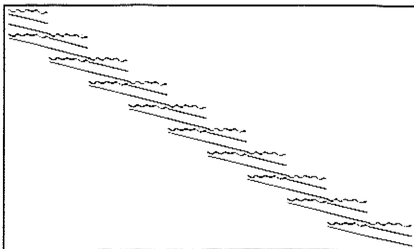
Picture for Problem 43 SCTAP3 Magnified 0.125
