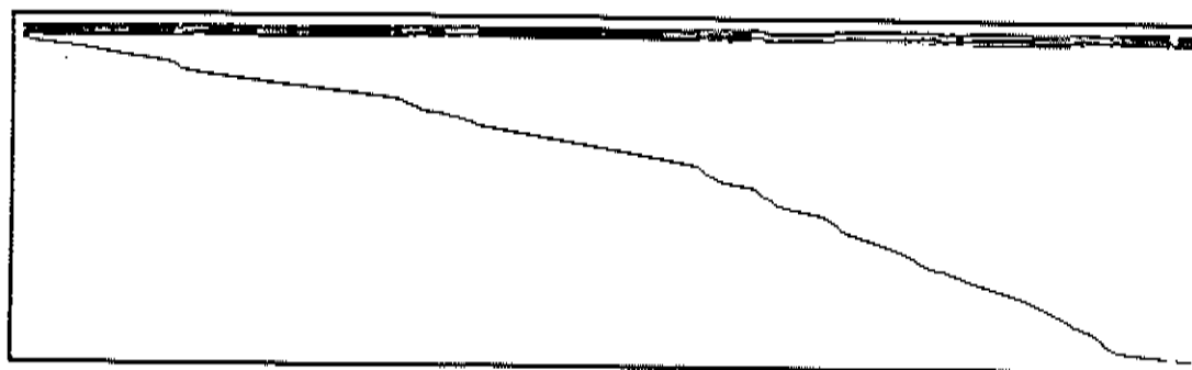
Picture for Problem 48 CZPROB Magnified 0.125
