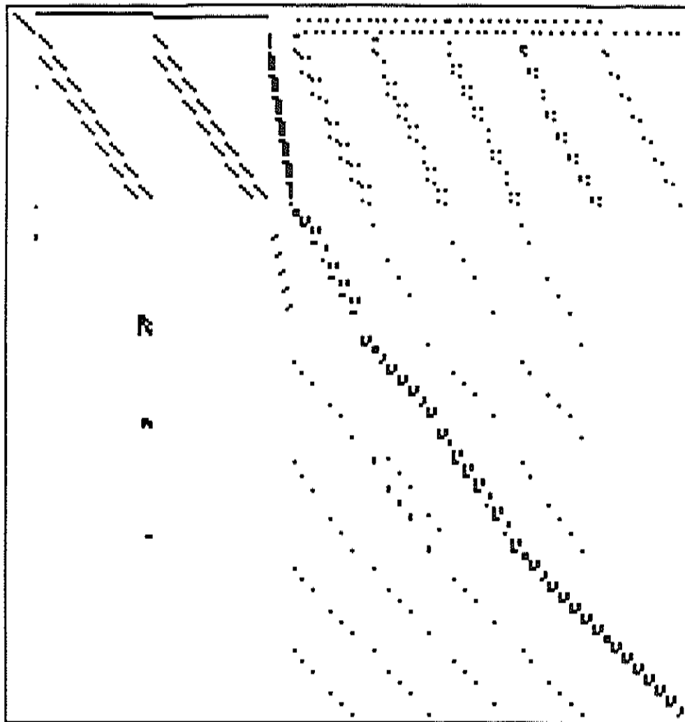
Picture for Problem 7 VTPBASE Magnified 2.0
