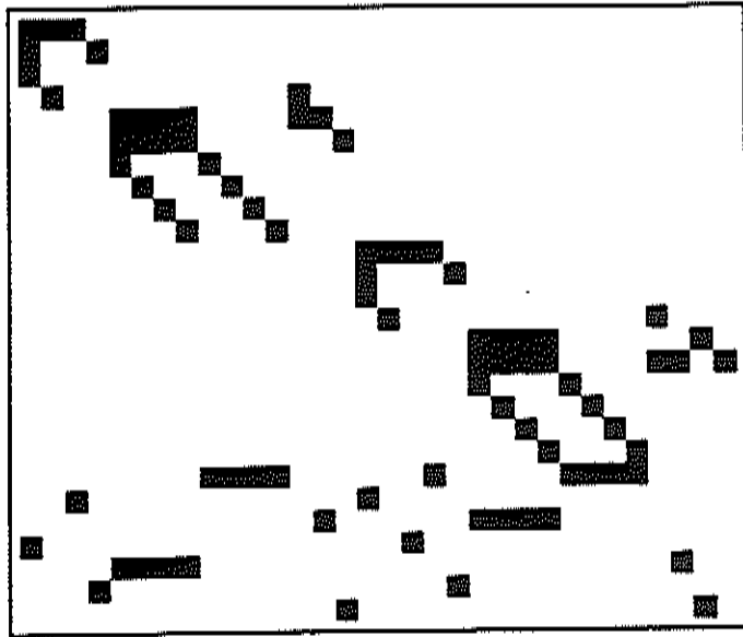
Picture for Problem 1 AFIRO Magnified 10.0
