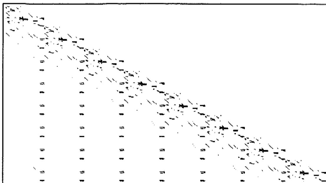
Picture for Problem 49 PILOTJA Magnified 0.25
