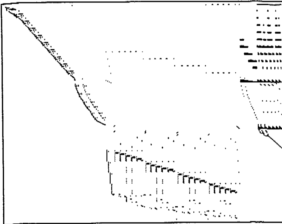
Picture for Problem 11 CAPRI Magnified 1.0
