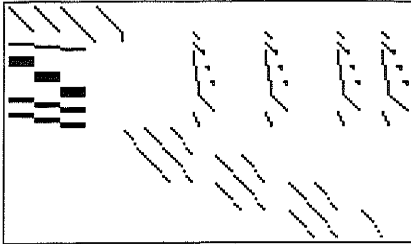
Picture for Problem 6 RECIPE Magnified 2.0
