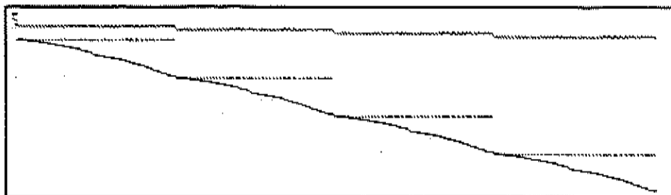
Picture for Problem 33 SHIP04S Magnified 0.25
