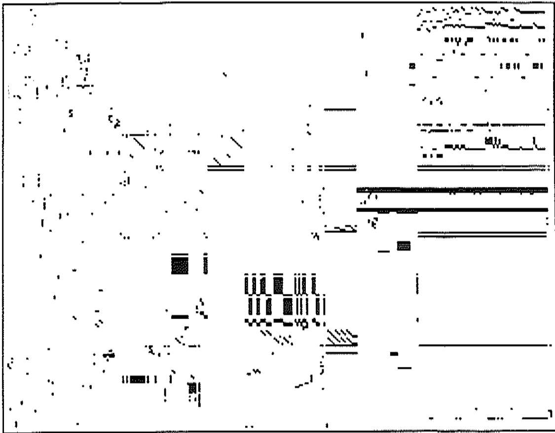
Picture for Problem 20 E226 Magnified 1.5
