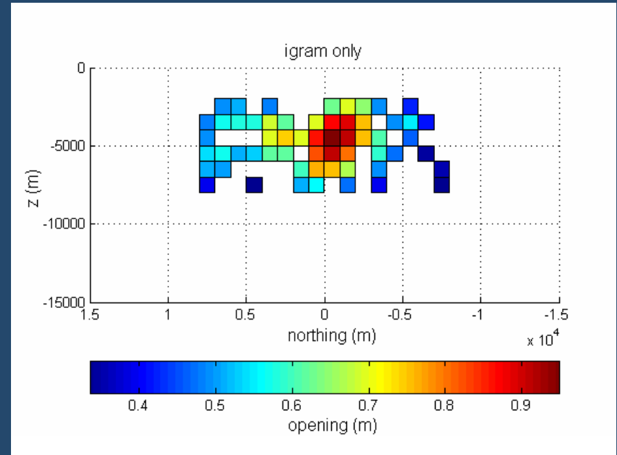
Estimate: Surface deformation only
