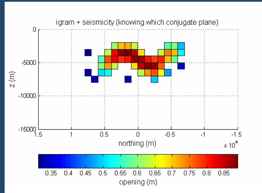
Estimate: Surface deformation + Seismicity – conjugate plane known
