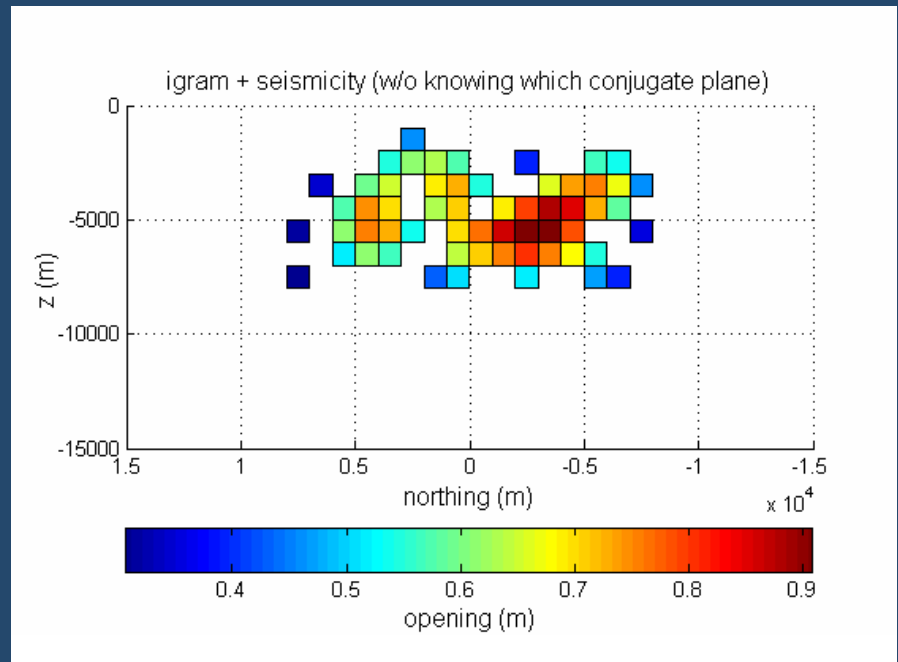
Estimate: Surface deformation + Seismicity – conjugate plane ambiguity
