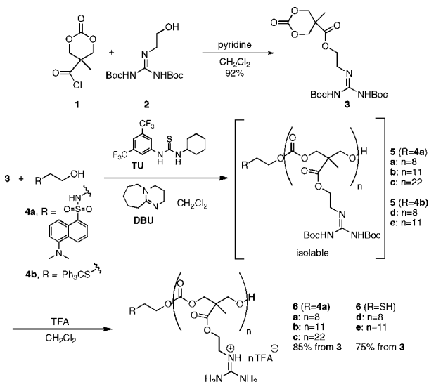
Scheme 1. Oligomerization Strategy
