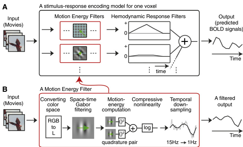
Figure 1. Schematic Diagram of the Motion-Energy Encoding Model
