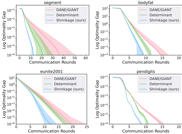
Figure 3: Experiments with real data for distributed Newton’s method applied to ridge regression. Line search is used in all methods to determine the step sizes. Number of total samples is rounded down to a multiple of the number of agents and split evenly to each agent. We let m = 100, \lambda = 0.1 for segment, m = 20, \lambda = 0.05 for bodyfat, m = 20, \lambda = 0.5 for eunite2001, m = 100, \lambda = 0.01 for pendigits, where \lambda is the regularization parameter and m denotes the number of agents.
