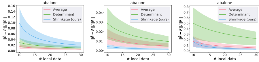
Figure 10: Sketched real data experiments for small regularizer regime. We use sketching matrix with entry i.i.d. \mathcal{N}(0, \frac{1}{m}) , sketch size m = 10000 . We use \Sigma = \frac{1}{n}A^T A . We take regularizer \lambda = 1 in the first two plots and \lambda = 0.001 in the third plot. \frac{md}{n} is used in replace of \frac{md_\lambda}{n} in the first plot and the third plot. \frac{md_\lambda}{n} is used in the second plot.
