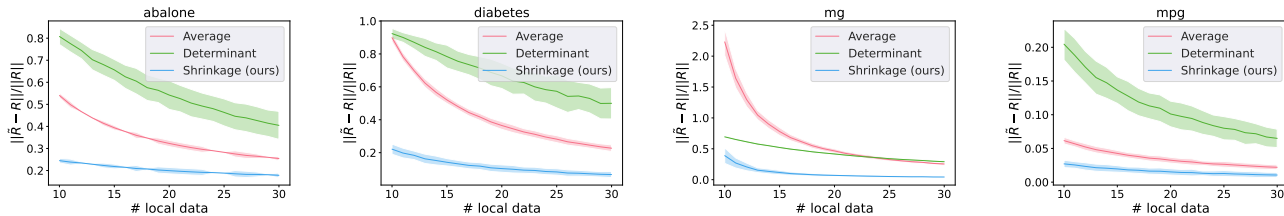
Figure 2: Experiments with real data in covariance resolvent estimation. The dataset is split evenly to each agent. We let \lambda = 0.001 and \Sigma = \frac{1}{n}A^T A . The relative matrix spectral norm difference between true covariance resolvent R and estimated covariance resolvent \tilde{R} is plotted, see Section 5.2 for details.
