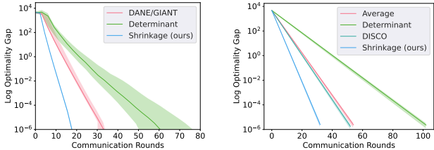
Figure 1: Synthetic data experiments on ridge regression. Total number of data n = 30000 , data dimension d = 150 , number of agents m = 200 , regularizer \lambda = 0.01 . The left plot shows the convergence of distributed Newton’s method (Algorithm 1). The right plot shows the convergence of our distributed preconditioned conjugate gradient method (Algorithm 2). Step-sizes are chosen via line search in all methods. See Section 5 for details.
