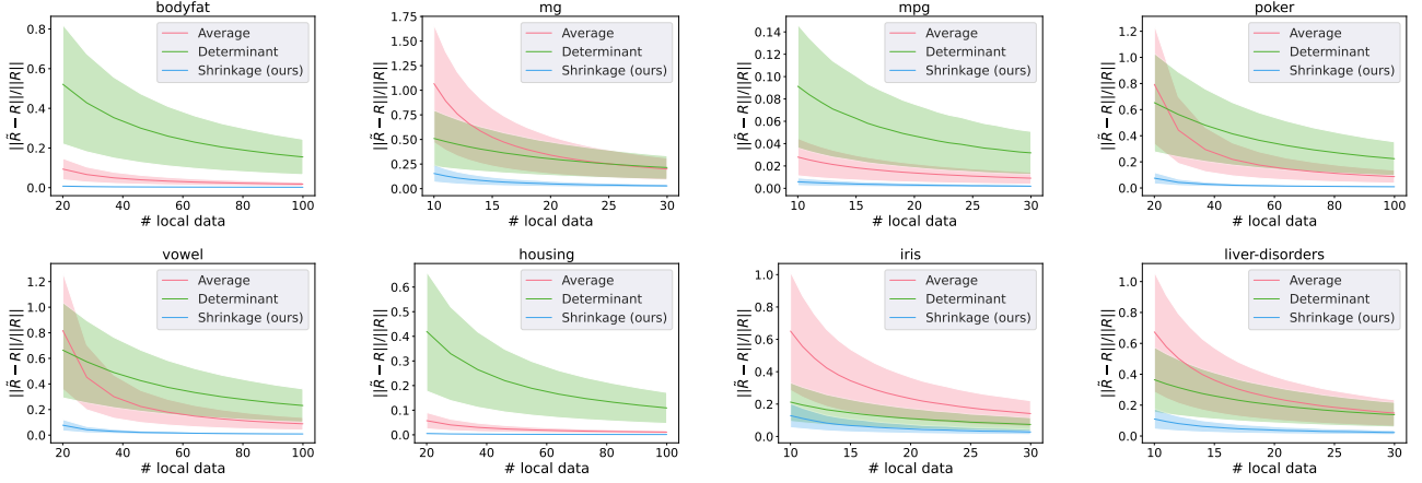
Figure 8: Sketched real data experiments for covariance resolvent estimation. We use sketching matrix with entry i.i.d. \frac{1}{\sqrt{n}}U(-\frac{\sqrt{12}}{2}, \frac{\sqrt{12}}{2}) , sketch size m = 10000 , regularizer \lambda = 0.001 . We use \Sigma = \frac{1}{n}A^T A .
