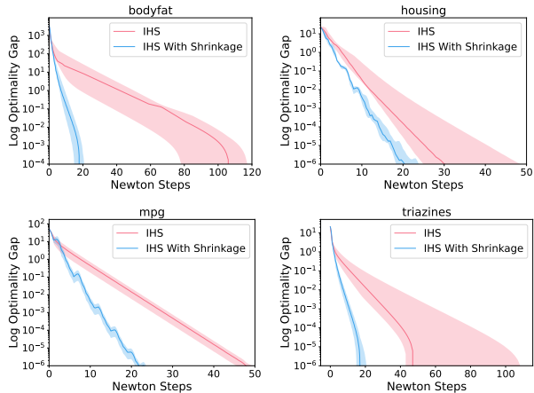
Figure 4: Experiments with real data for Iterative Hessian Sketch method applied to ridge regression. Line search is used to determine the step-sizes. We let \lambda = 0.01 for bodyfat, housing, mpg and \lambda = 0.001 for triazines; m = 100 for bodyfat, m = 50 for housing, m = 30 for mpg, m = 300 for triazines where \lambda denotes the regularization parameter and m denotes the sketch size.
