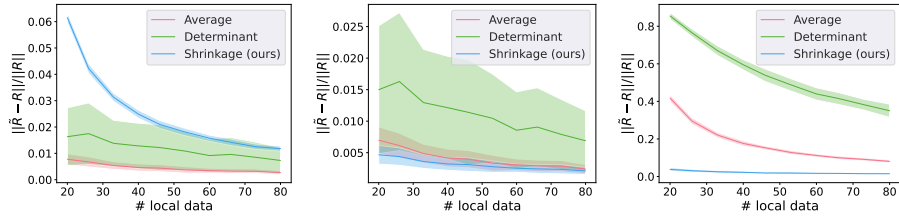
Figure 9: Synthetic data experiments for small regularizer regime. We experiment with m = 100 agents and data dimension d = 10 . Data is i.i.d. \mathcal{N}(0, \Sigma) , \Sigma = 100C^T C , C_{ij} \sim U(0, 1) . We take regularizer \lambda = 2000 in the first two plots and \lambda = 1 in the third plot. \frac{md}{n} is used in replace of \frac{md_\lambda}{n} in the first plot and the third plot. \frac{md_\lambda}{n} is used in the second plot.
