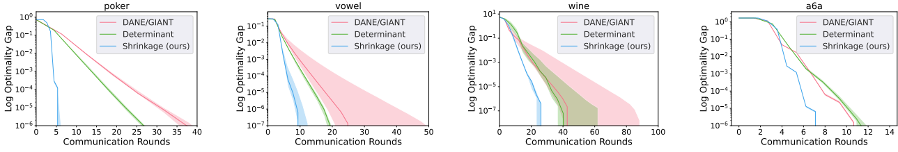
Figure 11: Normalized real data experiments for distributed Newton’s method for ridge regression. Number of total data is rounded down as multiple of number of agents and number of local data is number of total data divided by number of agents. Let \lambda denote the regularizer and m denote the number of agents. We pick m = 1000, \lambda = 0.001 for poker, m = 20, \lambda = 0.05 for vowel, m = 10, \lambda = 0.01 for wine, m = 50, \lambda = 0.5 for a6a.
