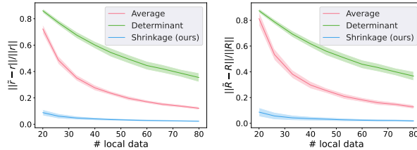
Figure 5: Synthetic data experiments for covariance resolvent estimation. Let m denote the number of agents, d denote data dimension, and \lambda denote the regularizer. We take m = 100 , d = 10 , \lambda = 0.1 . Data is i.i.d. \mathcal{N}(0, \Sigma) with \Sigma = 0.1I in the left plot, and \Sigma = 100C^T C , C_{ij} \sim U(0, 1) in the right plot.
