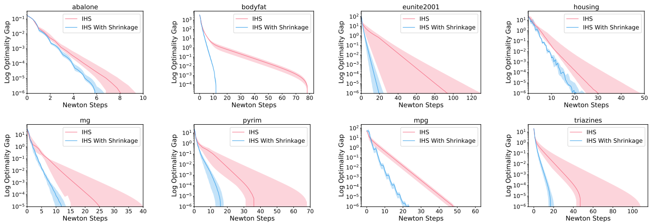
Figure 15: Real data experiments for Iterative Hessian Sketch method with exact shrinkage coefficient for ridge regression. Same parameter choice as in Figure 14.
