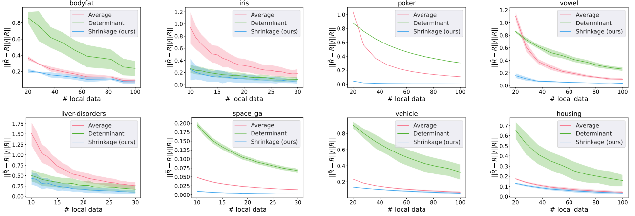
Figure 6: Normalized real data experiments for covariance resolvent estimation. \lambda = 0.001 . Number of total data is rounded down as multiple of number of local data, number of agent is number of total data divided by number of local data. We use \Sigma = \frac{1}{n} A^T A .
