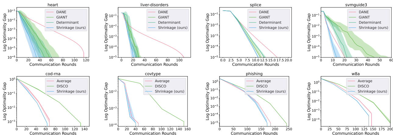
Figure 13: Normalized real data experiments for distributed second-order optimization algorithms for logistic regression. Top four plots are for distributed Newton’s method and bottom four plots are for distributed inexact Newton’s method. Number of total data is rounded down as multiple of number of agents and number of local data is number of total data divided by number of agents. For each Newton’s step, a refreshed data batch containing the number of local data divided by max_iters pieces of data is used (we limit number of Newton’s step to not exceed max_iters). Let \lambda denote the regularizer and m denote the number of agents. We pick m = 5, \lambda = 0.01, \text{max\_iters} = 20 for heart, m = 2, \lambda = 0.01, \text{max\_iters} = 10 for liver-disorders, m = 3, \lambda = 0.1, \text{max\_iters} = 5 for splice, m = 10, \lambda = 0.1, \text{max\_iters} = 20 for svmguide3, m = 100, \lambda = 1e - 5, \text{max\_iters} = 50 for cod-rna, m = 200, \lambda = 1e - 5, \text{max\_iters} = 50 for covtype, m = 40, \lambda = 0.01, \text{max\_iters} = 50 for phishing, m = 50, \lambda = 0.1, \text{max\_iters} = 50 for w8a.
