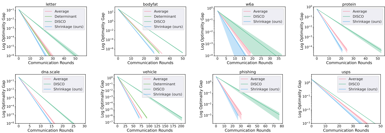
Figure 12: Normalized real data experiments for distributed inexact Newton’s method for ridge regression. Number of total data is rounded down as multiple of number of agents and number of local data is number of total data divided by number of agents. Let \lambda denote the regularizer and m denote the number of agents. We pick m = 1000, \lambda = 0.1 for letter, m = 20, \lambda = 0.01 for bodyfat, m = 30, \lambda = 1 for w6a, m = 50, \lambda = 0.1 for protein and usps, m = 50, \lambda = 10 for dna.scale, m = 40, \lambda = 1 for vehicle, m = 200, \lambda = 0.01 for phishing.
