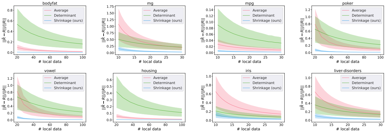
Figure 7: Sketched real data experiments for covariance resolvent estimation. We use sketching matrix with entry i.i.d. \mathcal{N}(0, \frac{1}{m}) , sketch size m = 10000 , regularizer \lambda = 0.001 . We use \Sigma = \frac{1}{n} A^T A .
