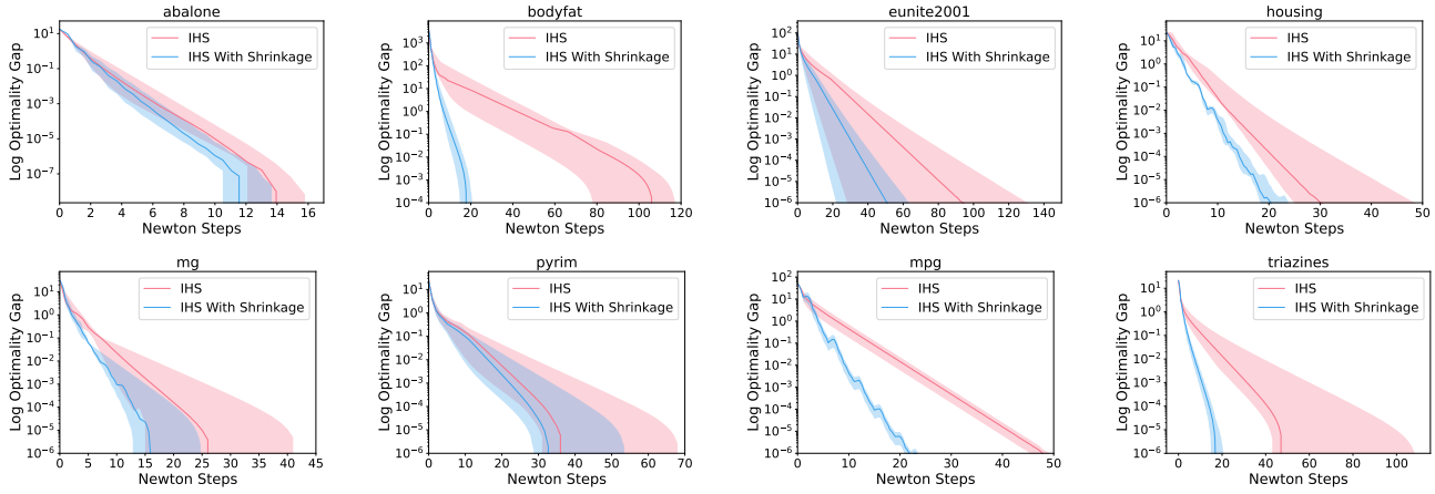
Figure 14: Real data experiments for Iterative Hessian Sketch method with heuristic shrinkage coefficient for ridge regression. Let \lambda denote the regularizer and m denote the sketch size. We pick \lambda = 0.001 for abalone, triazines and \lambda = 0.01 for bodyfat, eunite2001, housing, mg, pyrim, mpg. We pick m = 50 for abalone, m = 100 for bodyfat and pyrim, m = 300 for eunite2001, housing, and triazines, m = 20 for mg, and m = 30 for mpg.
