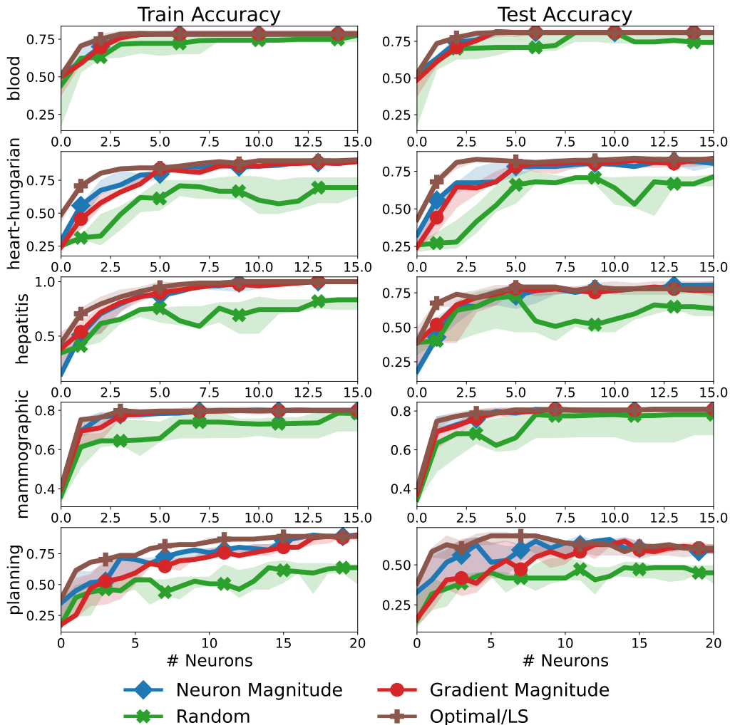
Figure 5. Pruning neurons on five additional datasets from the UCI repository. See Figure 2 for details. Our method ( Optimal/LS ) preserves test accuracy for longer than the baseline methods, leading to compact models with better generalization.
