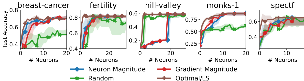
Figure 2. Pruning neurons from two-layer ReLU networks on binary classification tasks from the UCI repository. We compare our theory-inspired approach ( Optimal/LS ), against removing the neuron with smallest \ell_2 norm ( Neuron Magnitude ), removing the neuron with the smallest weighted gradient norm ( Gradient Magnitude ), and random pruning ( Random ). For Optimal/LS, we use Algorithm 2, which begins with optimal pruning and then switches to a least-squares heuristic. We plot test accuracy against number of active neurons. Optimal/LS dominates the baseline methods on every dataset and leads to improved test accuracy on breast-cancer and fertility .
