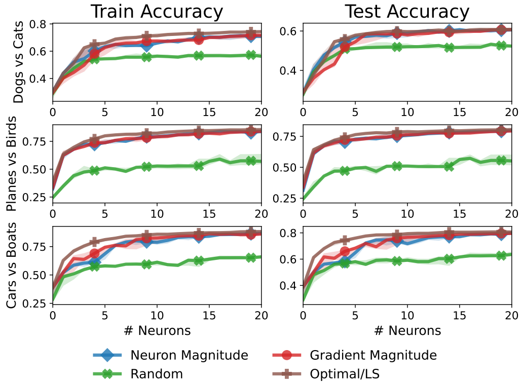
Figure 6. Pruning experiments on binary classification tasks from the CIFAR-10 dataset. This figure reproduces results from Figure 3 with training accuracies added and also includes results for an additional task, cats vs dogs, not presented in the main paper.
