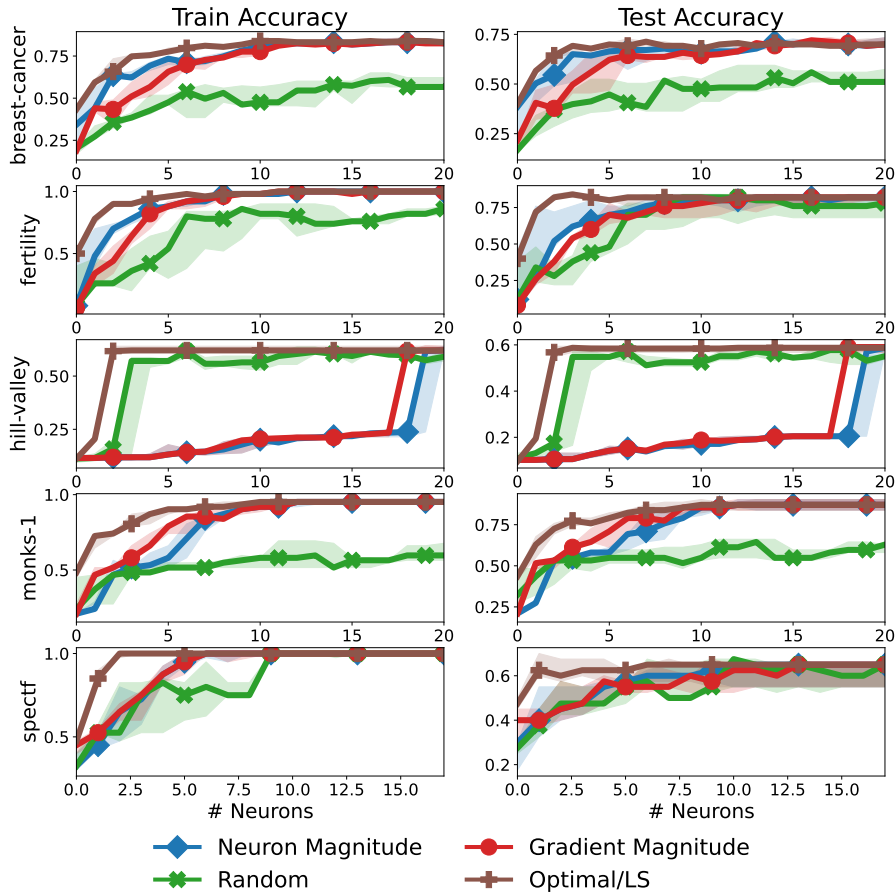
Figure 4. Pruning neurons on five datasets from the UCI repository. This figure extends Figure 2 with training accuracy in addition to the test accuracies shown in the main paper.
