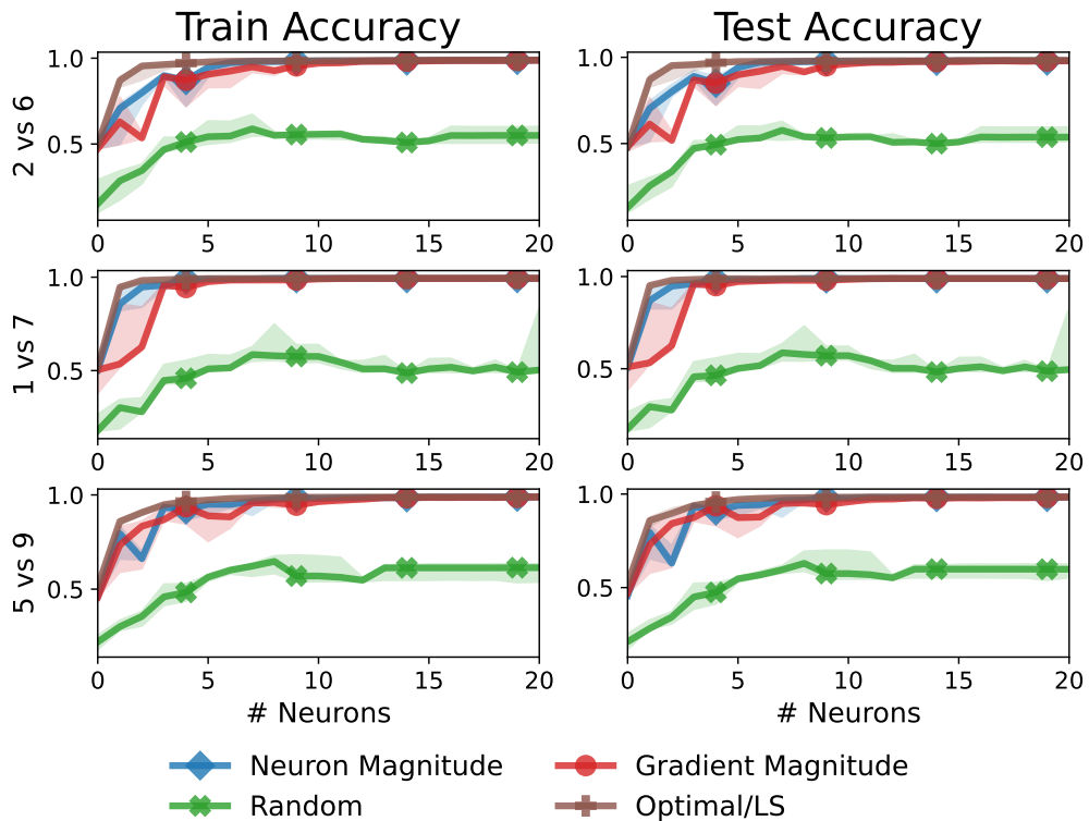
Figure 7. Pruning experiments on three binary classification tasks taken from MNIST.
