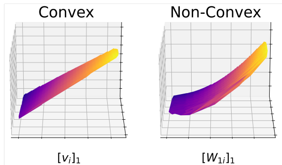
Figure 1. Convex vs non-convex solution spaces for two-layer ReLU networks. We plot the first feature of three different neurons; the non-convex parameterization maps the compact polytope of solutions for the convex parameterization into a curved manifold.
