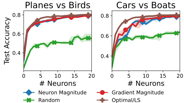
Figure 3. Pruning neurons from two-layer ReLU networks on two binary classification tasks drawn from the CIFAR-10 dataset. We compare our method ( Optimal/LS ) against baselines; see Figure 2 for details. Our approach, which makes use of a weight correction after pruning, outperforms every baseline.
