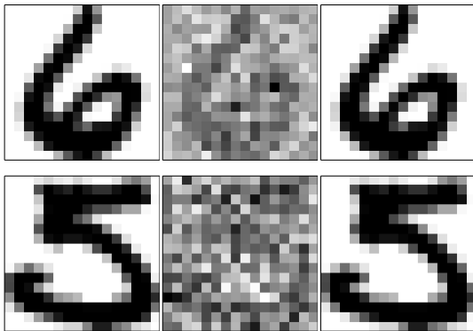
Left: true image. Middle: spectral initialization. Right: solution.
