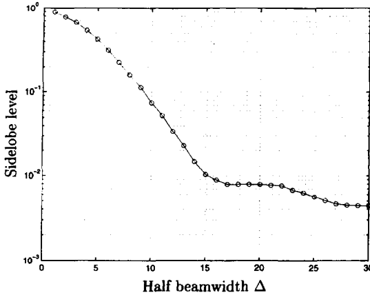
Fig. 2. Optimal tradeoff curve of sidelobe level versus half-beamwidth \Delta .
