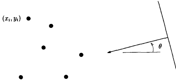
Fig. 1. Antenna array. A plane wave is incident from angle \theta . The output of the i th antenna element, located at (x_i, y_i) , is scaled by the complex weight w_i and added to the other scaled outputs. Constructive and destructive interference yields a combined output that is a function of the incidence angle.
