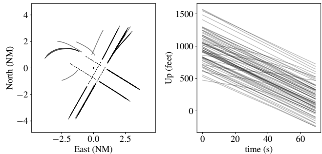
Fig. 7. Model for landings at JFK with K = 70 . Left, lateral view of archetypal trajectories. Right, archetypal trajectories vertical profile. Many of the archetypal trajectories overlap in lateral view but not in vertical profile. Each center corresponds to a slightly different glide slope.
