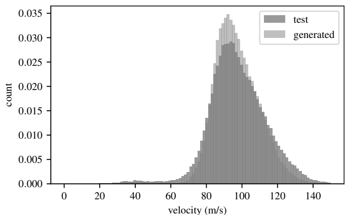
Fig. 15. Model for takeoffs at JFK with K = 50 . Histogram of lateral velocities for generated and held-out test data.
