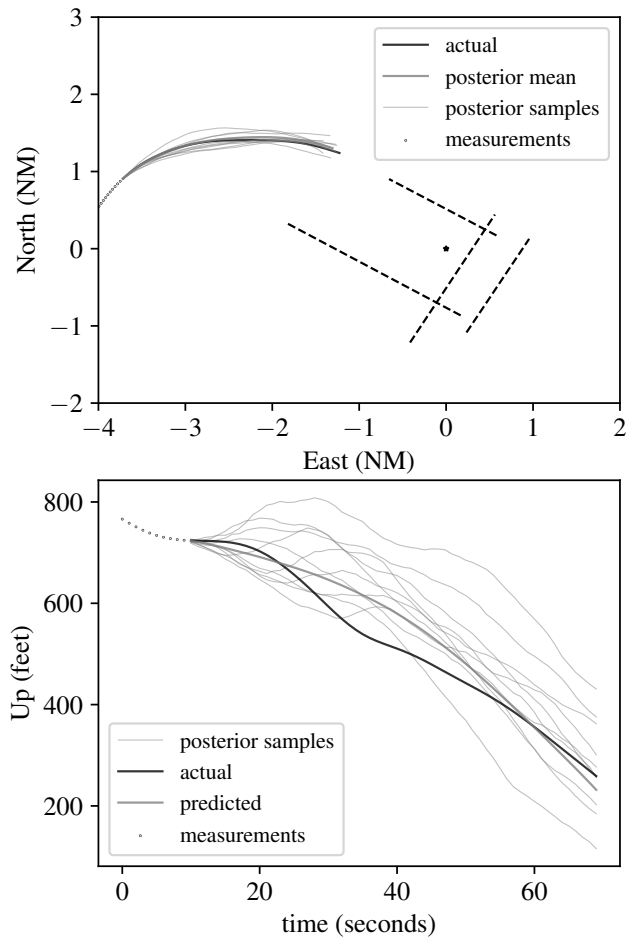
Fig. 14. Demonstration of inference for a JFK landing model with K = 20 . Given 10 samples (dots) of a landing trajectory (black), the model produces a prediction of where the aircraft will go (dark gray) and samples from the posterior distribution (light gray). The average RMS error for the prediction is 77.41 m.
