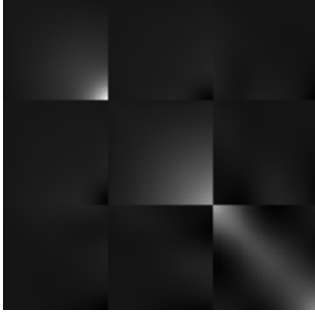
Fig. 4. Sample covariance matrix for the most probable cluster for takeoffs at JFK. Higher values of covariance are a lighter shade. The first third of the matrix corresponds to the east dimension, the second third corresponds to north dimension over time, and the final third corresponds to up dimension over time. Uncertainty increases with time, as aircraft are more likely to deviate from their nominal path later in the takeoff maneuver.
