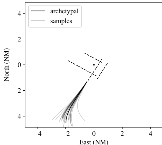
Fig. 6. Samples from the most probable cluster takeoff model at JFK with K = 20 . The cluster covariance naturally captures plausible takeoffs at JFK.
