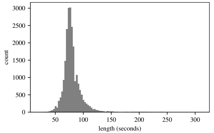
Fig. 2. Histogram of the length of takeoff trajectories at KJFK in seconds. The median is 70 seconds.
