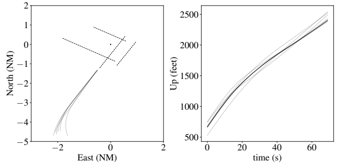
Fig. 5. Archetypal trajectory (black) and top-5 principal deviations (gray) for the most probable cluster of the model for takeoffs at JFK with K = 20 .
