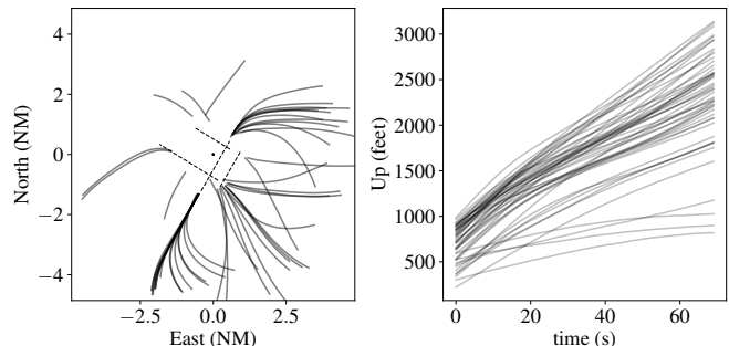
Fig. 8. Model for takeoffs at JFK with K = 50 . Left, archetypal trajectories lateral view. Right, archetypal trajectories vertical profile. As with landings, each cluster corresponds to different climb rates.
