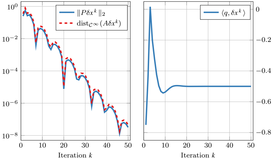
Fig. 3 Convergence of \{\delta x^k\}_{k \in \mathbb{N}} to a certificate of dual infeasibility for problem (32) with a = 0 , u_1 = 2 , and u_3 = +\infty
