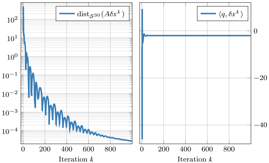
Fig. 6 Convergence of \{\delta x^k\}_{k \in \mathbb{N}} to a certificate of dual infeasibility for problem \text{inf}d1 from SDPLIB
