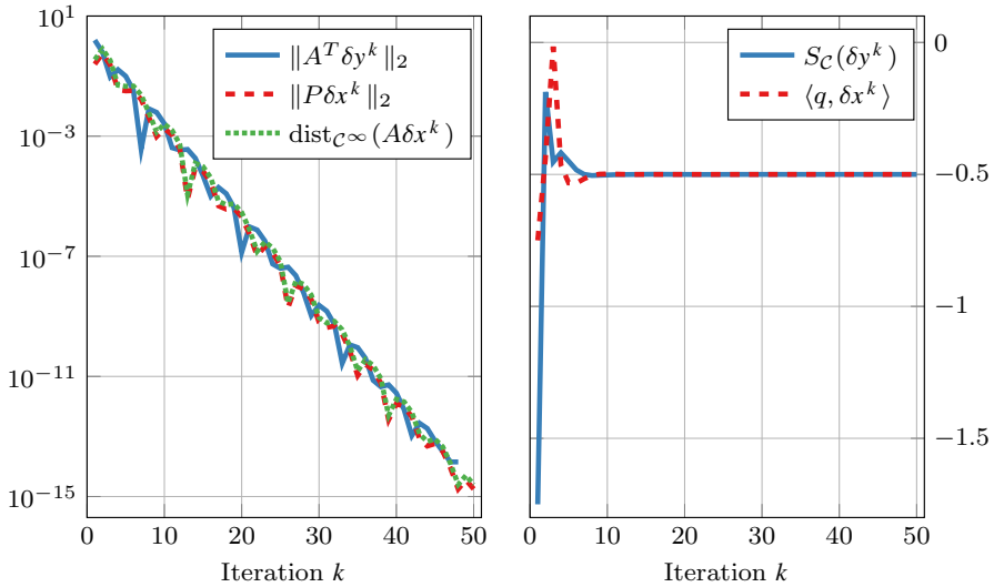
Fig. 4 Convergence of \{\delta y^k\}_{k \in \mathbb{N}} and \{\delta x^k\}_{k \in \mathbb{N}} to certificates of primal and dual infeasibility, respectively, for problem (32) with a = 0, u_1 = 0 and u_3 = +\infty
