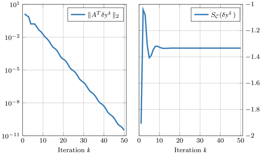
Fig. 2 Convergence of \{\delta y^k\}_{k \in \mathbb{N}} to a certificate of primal infeasibility for problem (32) with a = 1, u_1 = 0 and u_3 = 3
