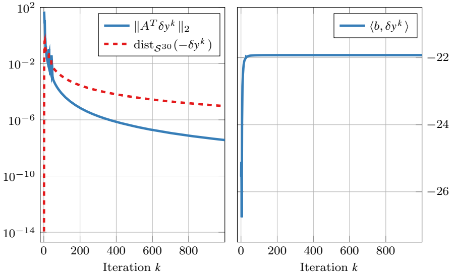
Fig. 5 Convergence of \{\delta y^k\}_{k \in \mathbb{N}} to a certificate of primal infeasibility for problem \text{inf}p1 from SDPLIB
