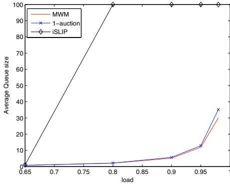
Fig. 3. Average queue sizes for MWM, 1-Auction and iSLIP.
