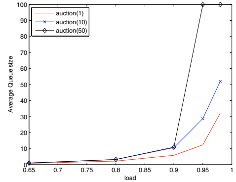
Fig. 5. Average queue sizes for auction(1), auction(10), auction (50)
