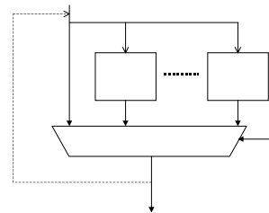
Fig. 3. A schematic for the implementation of APSARA. The old matching, S(t) , and the new arrivals, A(t + 1) , are used to compute the weights of the k neighbor matchings in parallel. The new matching, S(t + 1) , is the one with highest weight among all the neighbors. Note that this architecture is parallel and can be easily pipelined
