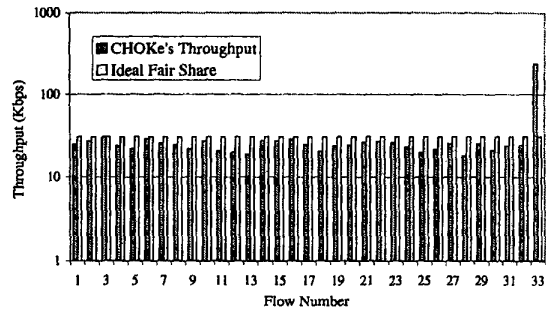
Fig. 4. CHOCe: Throughput Per Flow
